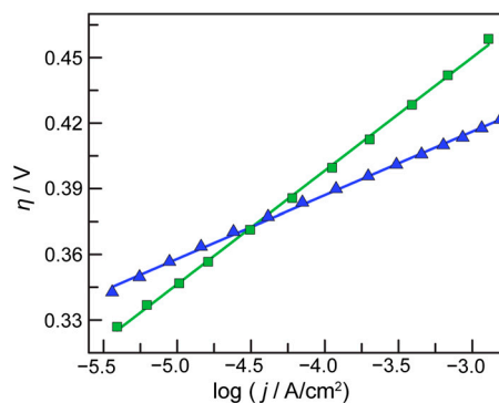
Fig. 2. Tafel plot, \eta = (V_{\text{app}} - iR - E^0) , of a Ni-B i -catalyst film operated in 0.5-M B i , pH 9.2 (blue triangles), and a Co-B i -catalyst film operated in 1-M B i , pH 9.2 (green squares). E^0 is the thermodynamic potential of water splitting under the conditions of the experiment, \eta is the overpotential, and iR accounts for the uncompensated cell resistance. The slopes of the linear fits to the data are 52 mV/decade and 29 mV/decade for Co-B i and Ni-B i , respectively.
