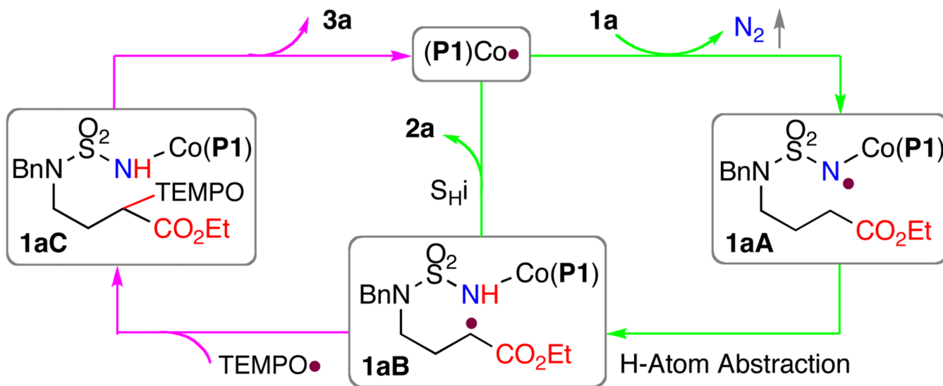
Scheme 3. TEMPO Trapping of Carbon-Based Radical Intermediate Involved in Radical Mechanism of Co(II)-Based Metalloradical C-H Amination.
