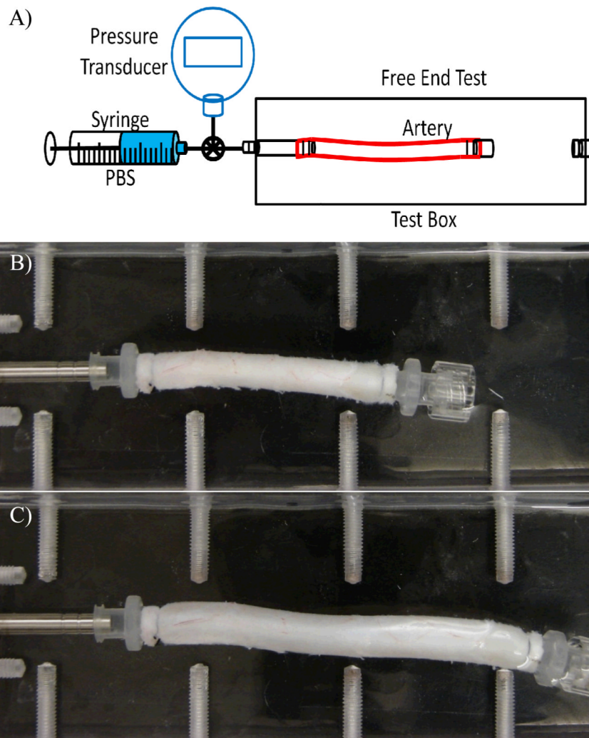
Figure 1. Top: Schematics of experimental setup for pressurized inflation test. Arteries are cannulated and pressurized with a syringe pump while one end is free to expand axially and circumferentially. Pictures: An artery during the test under a pressure of 0 mmHg (top) and 200 mmHg (bottom), respectively.
