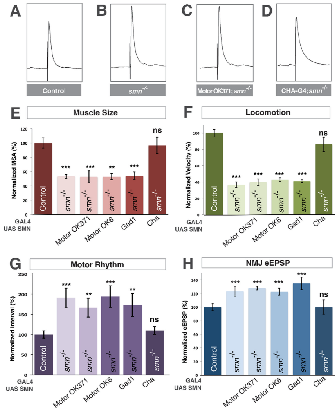
Figure 3. SMN expression is required in cholinergic neurons and not motor neurons
