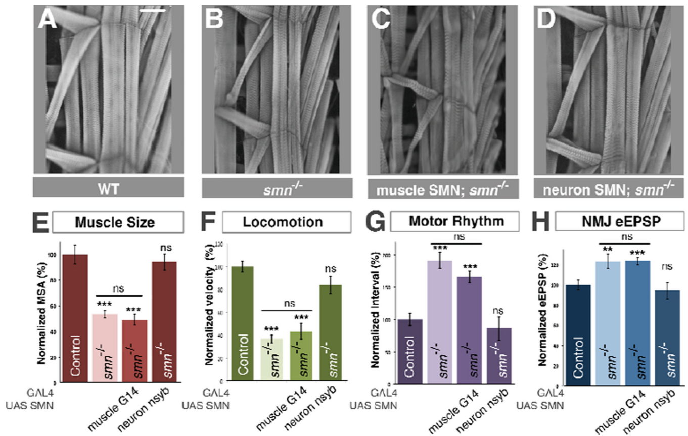
Figure 2. SMN expression is required in neurons but not muscles to rescue smn mutants A–D. Sample images of muscles from segment A3 of (A) control, (B) smn X7 mutant, (C) smn X7 mutants with transgenic SMN expression only in muscles (G14-Gal4/UAS::flagSMN; smn X7 / smn X7 ) or (D) neurons (nsyb-Gal4/UAS::flagSMN; smn X7 / smn X7 ). Restoration of SMN expression in muscles has no effect on muscle size however restoration in neurons fully rescues muscle surface area. E–H. Quantification of muscle surface area (E), locomotion (F), motor rhythm (G) and NMJ eEPSP amplitude (H) normalized to controls. Expression of transgenic SMN in neurons rescues all of smn mutant phenotypes while expression in muscles does not. Data are represented as mean \pm SEM, **= p < 0.01 , ***= p < 0.001 . See also Figure S2.
