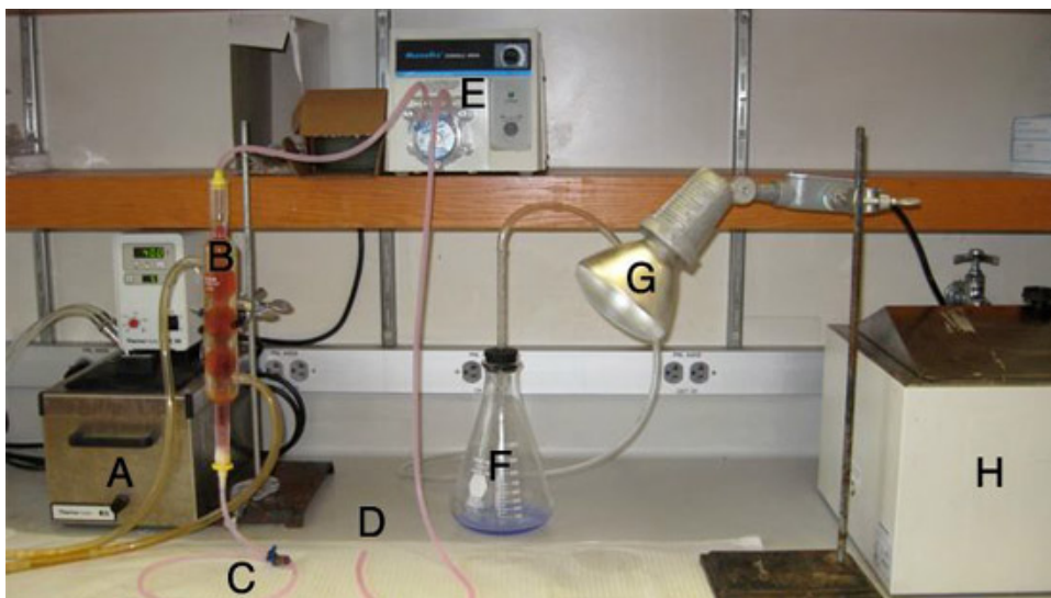
Figure 1. Perfusion set up. A. Water circulator for warming column. B. Column containing perfusion media. C. Stopcock controlling pump outflow. D. Pump inflow. E. Variable-speed peristaltic pump. F. Vacuum flask with Bio-Clean detergent. G. Heat lamp. H. Water bath for warming perfusion media.
