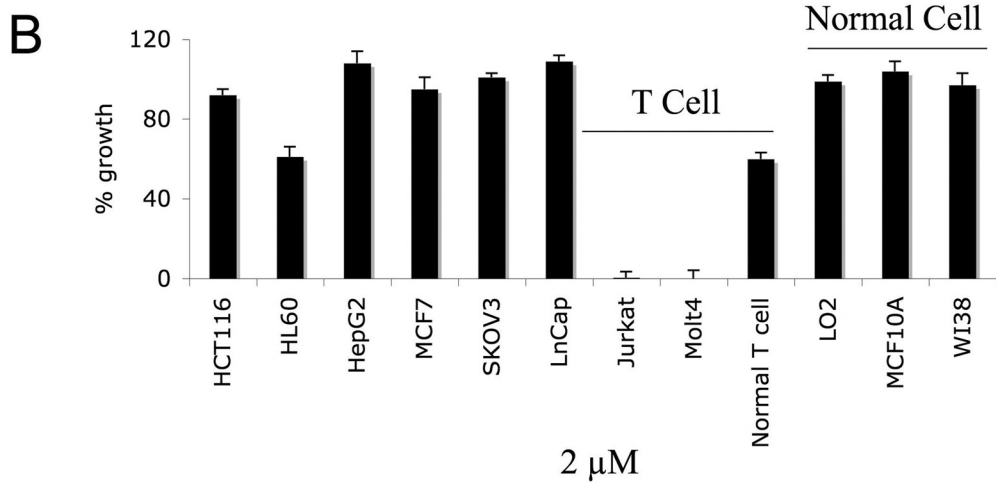
Fig. 3. Expression profile of Itk in 45 cell lines (41 cancer cell lines and 4 normal cell lines) and CTA056-induced growth inhibition of a panel of cancer cells. The expression profile of Itk was measured using Western blot (A). For growth inhibition, cells were seeded at 5000 cells/well in 96-well plate overnight and were treated with CTA056 (B, 0 and 2 μM; C, 0–10 μM). After 72 h, cell proliferation was measured using the MTT assay. Columns, mean; bars, S.D., n = 3.
