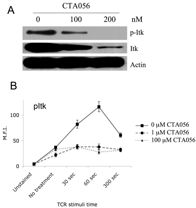
Fig. 6. Inhibition of Itk phosphorylation in Jurkat cells after treatment with CTA056. Itk phosphorylation in Jurkat cells was examined using Western blot (A). Cells were seeded at 10^6 cells/ml (5 ml) and treated with CTA056 at the indicated concentrations for 24 h. Before harvest, cells were pretreated with pervanadate for 15 min. pItk, Itk, and actin levels were measured using the corresponding antibodies through Western blot. B, Jurkat cells were pretreated with CTA056 30 min and then incubated with anti-CD3, anti-CD28 monoclonal antibodies ( 10 \mu\text{g/ml} ), and protein G ( 10 \mu\text{g/ml} ). At 30 s, 1 min, and 5 min, the stimulation was stopped. The cells were then permeabilized and stained with a phospho-Itk-specific antibody. One of three similar experiments is depicted. Values are averages of triplicate samples.
