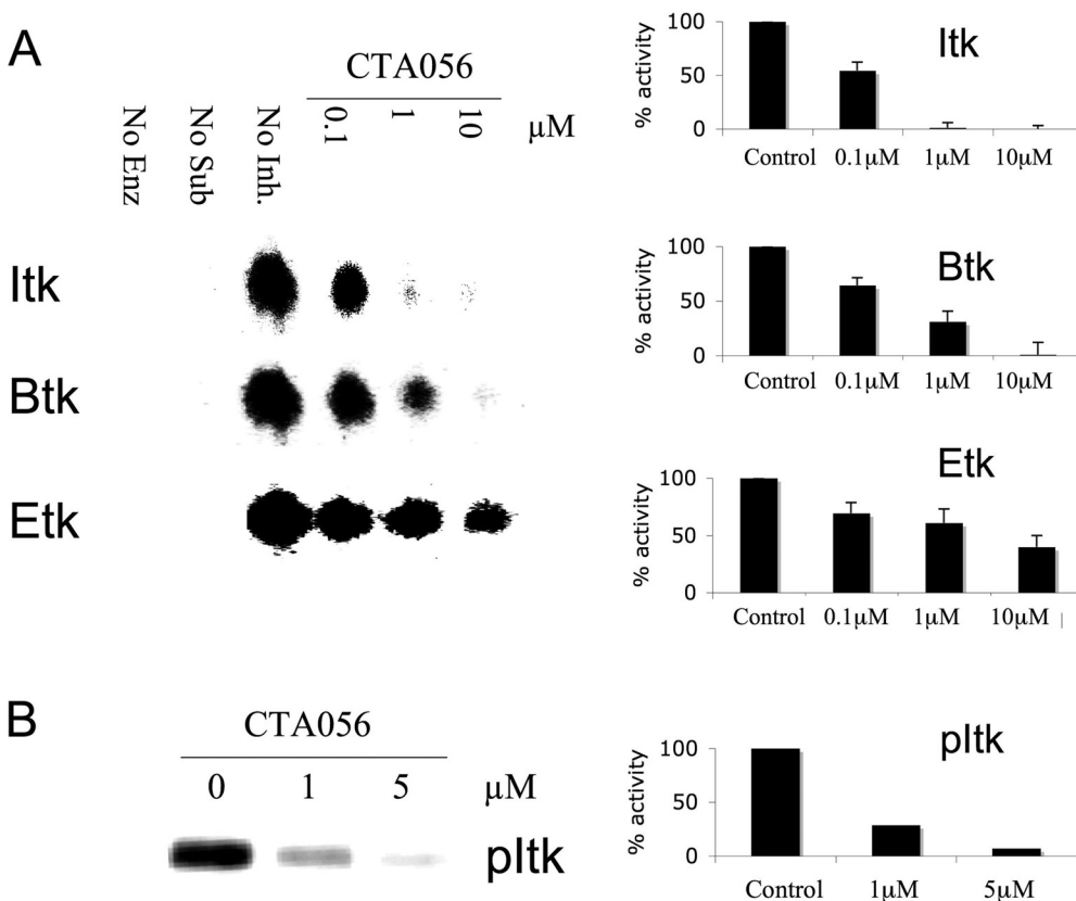
Fig. 2. Kinase inhibitory activity of CTA056 (A) and inhibition of Itk auto-phosphorylation by CTA056 (B). Kinase activity was measured using TLC assay. Purified kinase (20 nM), CTA056 (0–10 \mu M), and the peptide substrate were incubated with [ 33 P]ATP in a kinase reaction. The resulting product was analyzed on a TLC plate. The relative kinase activity to control was calculated using densitometry. Itk auto-phosphorylation activity was measured by an in vitro kinase assay. Purified Itk (100 ng) was mixed with CTA056 inhibitor, the ice-cold ATP and hot r-[ 33 P]ATP in the kinase assay buffer, and the Itk auto-kinase activity was analyzed by filmless autoradiographic analysis (Bio-Rad Laboratories). Columns, mean; bars, S.D., n = 3.
