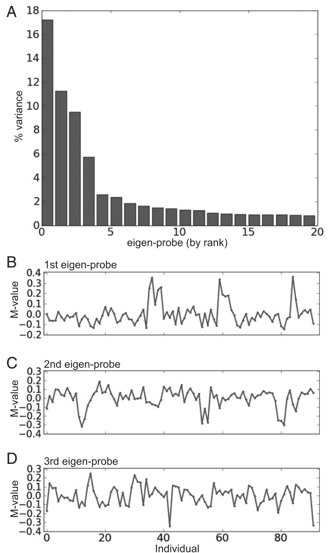
Fig. 4. PCA revealed covariant DNA methylation patterns in a population. (A) Percentage of variation in DNA methylation accounted for by the top 20 eigen-probes. (B–D) DNA methylation signatures for the top 3 eigen-probes over the population of individuals. Using a methylation variation (M-value) cutoff of \pm 0.1 allowed us to create groups of correlated individuals for each eigen-probe that we could then test for enrichment for particular traits (main text).
