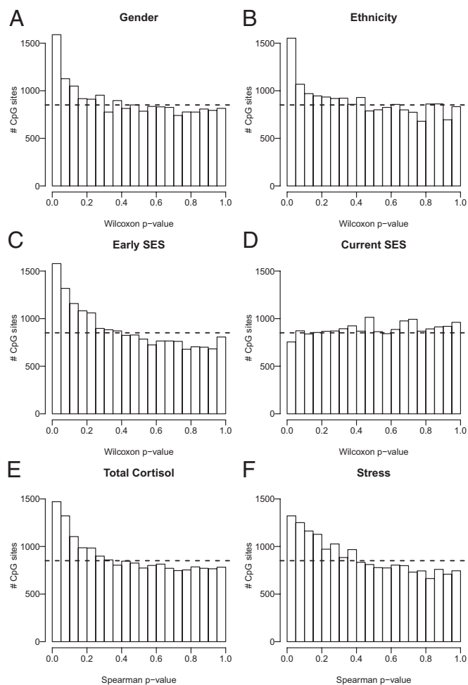
Fig. 2. Demographic and psychosocial factors were associated with DNA methylation. Graphical representations of P -value distributions. In each case, the dashed line represents the uniform distribution that was expected by chance. The skewed distributions with an enrichment of CpG sites having small P values suggested that sex (A), ethnicity (B), and early-life SES (C) were correlated with DNA methylation. (D) This contrasted with the lack of correlation suggested by the uniform P -value distribution of current SES. Furthermore, cortisol output (E) and perceived stress (F) were both correlated with DNA methylation. Testing for correlations was done using either Wilcoxon tests (A–D) or Spearman \rho statistics (E and F).
