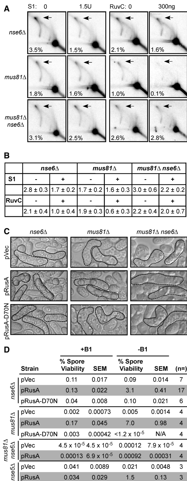
Figure 6. nse6Δ Mutants fail in meiosis because of DNA joint molecule accumulation. (A) DNA prepared at 4.5 or 5 h ( nse6Δ and mus81Δ ) or 6 h ( nse6Δ mus81Δ ) after meiotic induction was digested with Pvu II and treated with the indicated amounts of either the ss DNA-specific S1 nuclease or the purified RuvC and assayed by two-dimensional gel electrophoresis and Southern blot hybridization using the probe shown in Figure 3B. The percentage given is the amount of JMs, indicated by arrows, divided by the amount of total DNA. All
