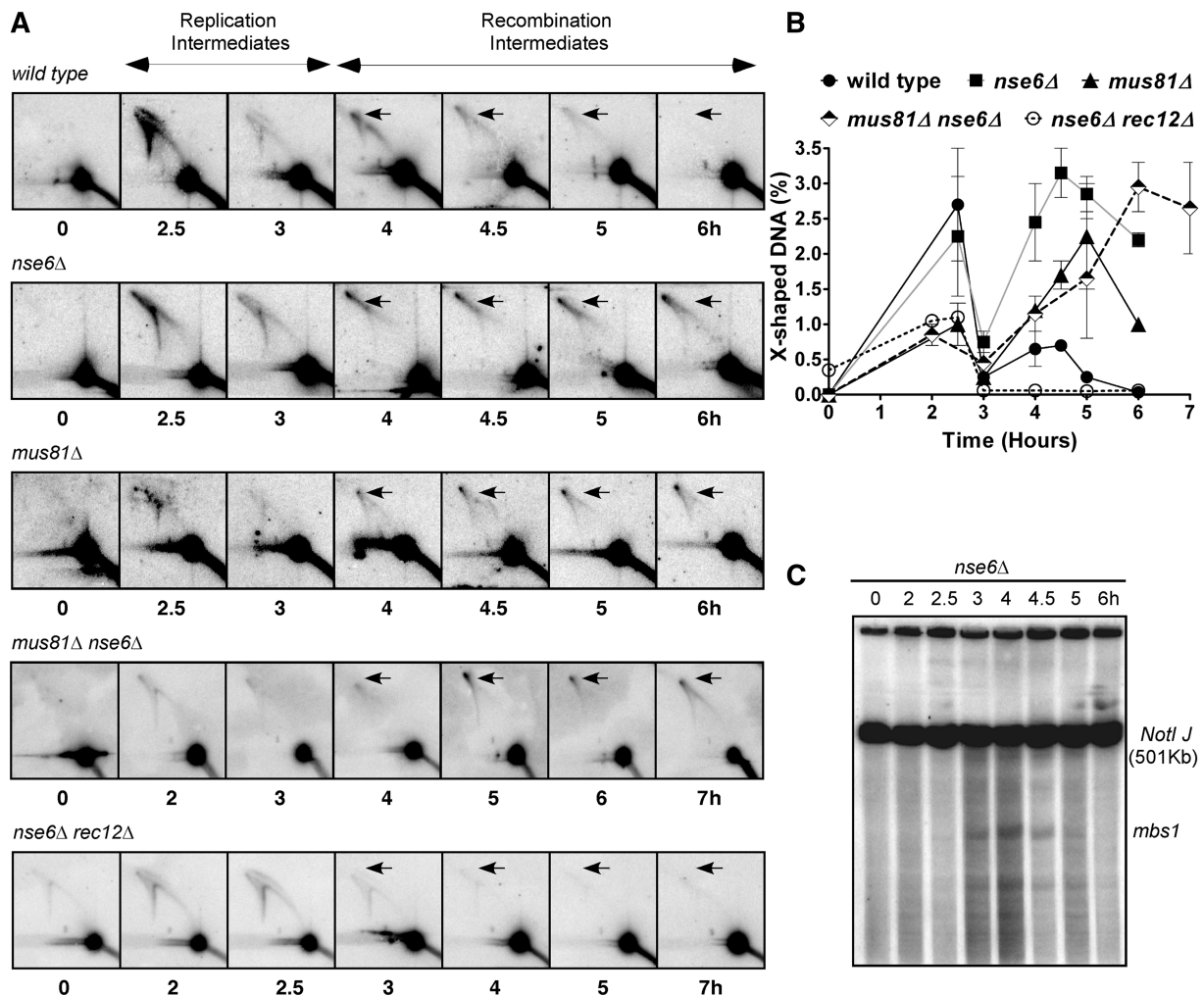
Figure 4. Joint molecules accumulate during meiosis in the nse6Δ mutant. (A) Diploid pat1-114 wild-type (GP6656), nse6Δ (GP6234), mus81Δ (GP6657) and nse6Δ mus81Δ (GP7765) and haploid pat1-114 nse6Δ rec12Δ (GP7773) strains were induced for meiosis. DNA was extracted at the time indicated and digested with PvuII to generate 11.2 kb DNA fragments containing mbs1 (Figure 3B). Branched DNA molecules were assayed by two-dimensional gel electrophoresis (8,88) in which the first dimension slowly separates DNA primarily by mass and the second dimension primarily by shape, as branched structures have less mobility than linear DNA, and subsequent Southern blot hybridization. DNA from 2.5–3 h shows branched DNA structures arising from replication, while at 4 h, the structures are primarily recombination intermediates (8). Note that X-shaped DNA (arrows) forms in the wild-type at 4 h and disappears by 6 h, as expected for HJs that form and are resolved during the repair of DSBs, but form and persist in nse6Δ , mus81Δ and nse6Δ mus81Δ mutants. (B) Quantification of the X-shaped DNA observed in (A). Each datum is the mean of two independent experiments, with the error bars indicating the range. (C) Meiotic DSBs arise and disappear with wild-type timing in a diploid nse6Δ strain GP6234. DNA prepared at the indicated time after induction of meiosis was digested with NotI , separated by pulsed-field gel electrophoresis and analyzed by Southern blot hybridization with a probe specific to the left end of the 501 kb NotI fragment J, which contains mbs1 near its middle. Note that DSBs appear after replication at 3 h, reach a maximum at 4 h and are mostly repaired by 5 h, consistent with previous results from wild-type and mus81Δ strains (8,9,68,69) and with the timing of HJ formation observed in (A).
