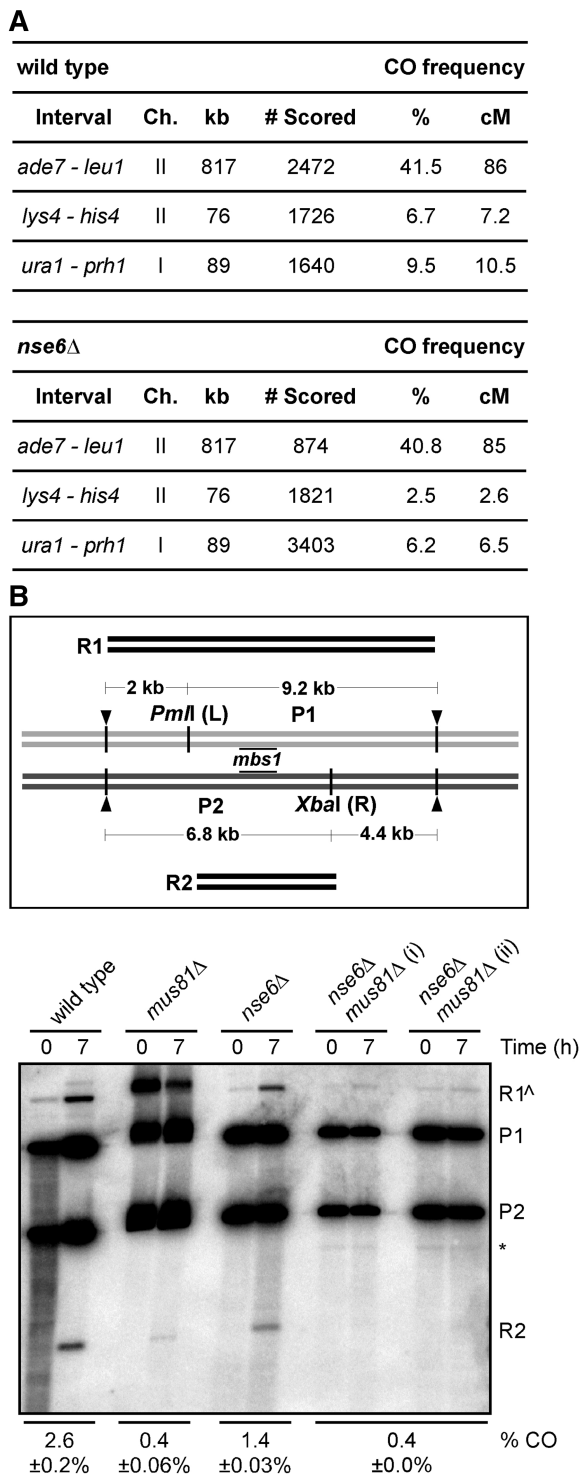
Figure 3. Effect of nse6Δ mutation on the frequency of meiotic crossovers. (A) Crossover (CO) frequencies in three intervals in the wild-type and nse6Δ backgrounds. The percent of recombinant spore colonies was estimated to genetic distance in centimorgans with Haldane's equation. The number of colonies analyzed is the total from at least three independent experiments. (B) Amount of crossover DNA generated at the mbs1 hotspot (8). Diploid pat1-114 wild-type (GP6656), mus81Δ (GP6657), nse6Δ (GP6234) and nse6Δ mus81Δ (GP7765) strains with heterozygous restriction sites PmlI (L) and XbaI (R) flanking mbs1 were assayed. Digestion with these enzymes and PvuII (black arrowheads), which cuts outside L and R, gives two parental DNA fragments [9.2 kb (P1) or 6.8 kb (P2)] and two
