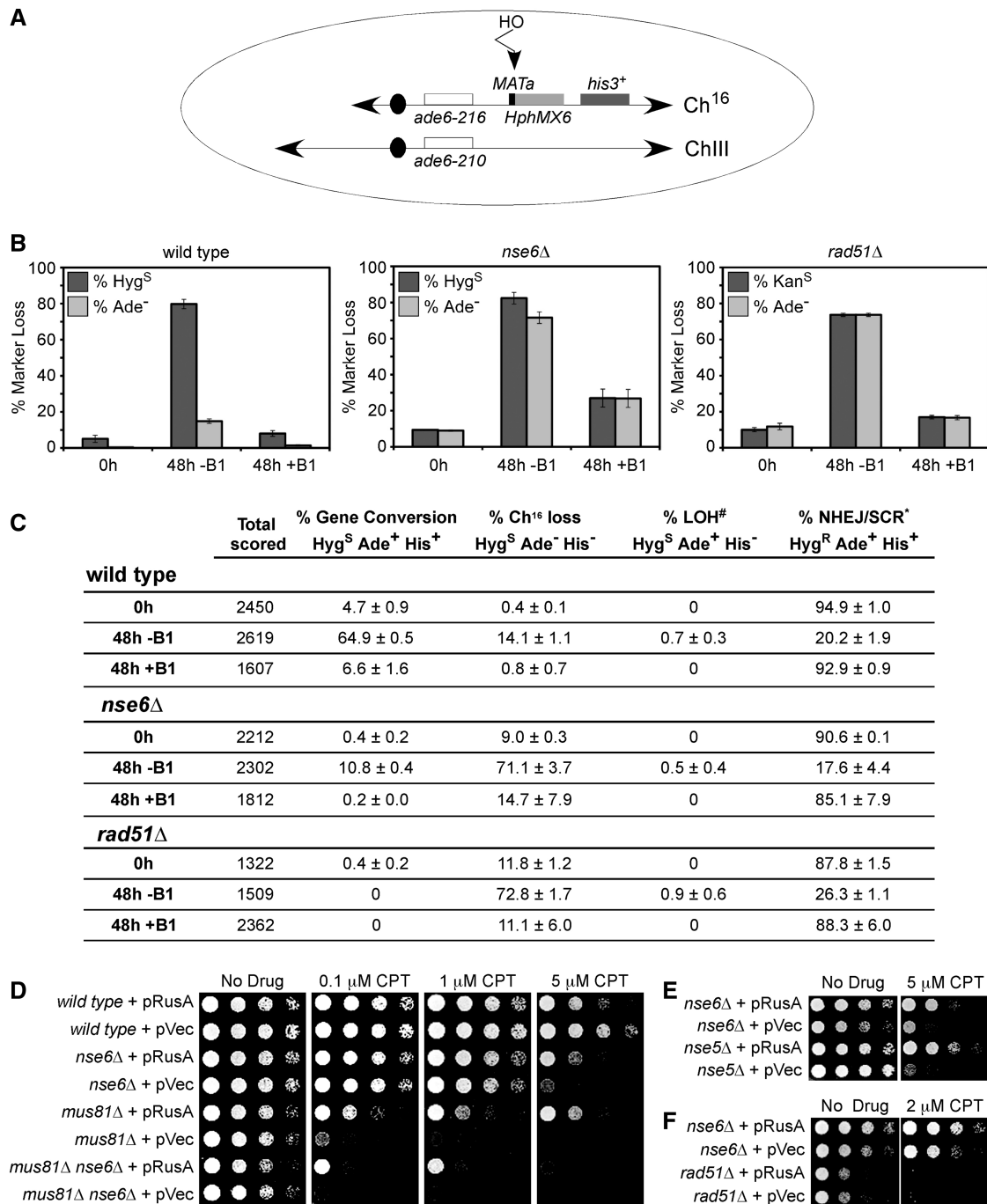
Figure 1. Mitotic roles for the Smc5–Smc6 complex. (A) Schematic of the HO-induced DSB minichromosome system. The minichromosome Ch 16 and full-length Ch III with their centromeric regions (black ovals), histidine marker his3 + (dark grey box) and complementing ade6 heteroalleles ( ade6-216 and ade6-210 (86); white boxes) are shown along with a MATa site for HO DSB formation (black rectangle) and the adjacent hphMX6 (hygromycin)-resistance marker (light gray box) for wild-type and nse6Δ cells. As rad51 was deleted using the hygromycin-resistance marker, a minichromosome bearing a kan (kanamycin)-resistance marker was used in this background. MATa is ~25 kb from the ade6 marker. Removal of thiamine (B1) derepresses the HO gene, whose product generates a DSB at the MATa target site (vertical arrowhead). HO-induced DSBs can result in (i) loss of Ch 16 with diagnostic Ade - and Hyg S phenotype, (ii) repair of the DSB by interchromosomal gene conversion using Ch III as a template, resulting in the loss of MATa and hphMX6 cassette and an Ade + and Hyg S phenotype or (iii) maintenance of the initial Ade + Hyg R phenotype, if the DSB is repaired by either non-homologous end-joining (NHEJ) or sister chromatid repair. The HO system can also assay levels of spontaneous minichromosome Ch 16 loss, by scoring marker loss in the absence of HO induction (0 h, and 48 h culturing in thiamine). (B) and (C) Genetic analysis of site-specific DSB repair in wild-type (left panel), nse6Δ (middle panel), and rad51Δ (right panel) backgrounds. Percentage marker loss is given for cells grown in repressive (0 h and 48 h, +B1) or derepressive media (48 h, -B1). Data are means and standard errors from three independent experiments. # Loss of heterozygosity (LOH) can occur through various mechanisms, as described in (58). *Sister chromatid repair (SCR) also results in a Hyg R Ade + phenotype. (D) RusA expression partially rescues the CPT sensitivity of nse6Δ , mus81Δ and nse6Δ mus81Δ mutants. (E) and (F) RusA expression partially rescues the CPT sensitivity of nse5Δ and nse6Δ , but does not rescue that of rad51Δ cells. (D–F) Five-fold serial dilutions of the indicated strains were plated onto medium that lacked thiamine to derepress plasmid-borne gene expression. Cells were either untreated or treated with the indicated concentrations of CPT and grown at 32°C for 3 days. pVec denotes an empty vector (87).
