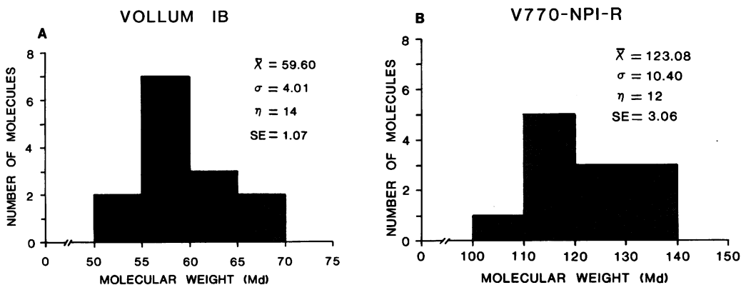
FIG. 3. Length distribution of Vollum 1B (A) and V770-NP1-R (B) plasmid molecules. Statistical parameters are shown for each graph.
