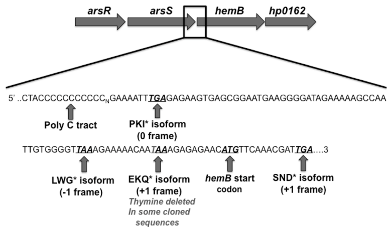
Figure 1. arsS polymorphisms and the arsRS operon
