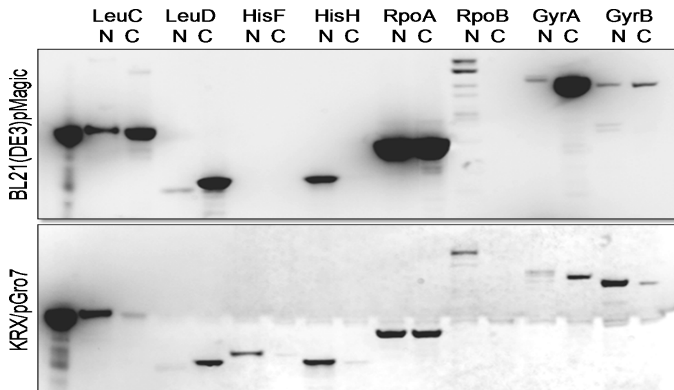
Fig. (2). Expression of E. coli proteins for protein-protein interactions. The HaloTag recombinant proteins were visualized with TMR ligand.
