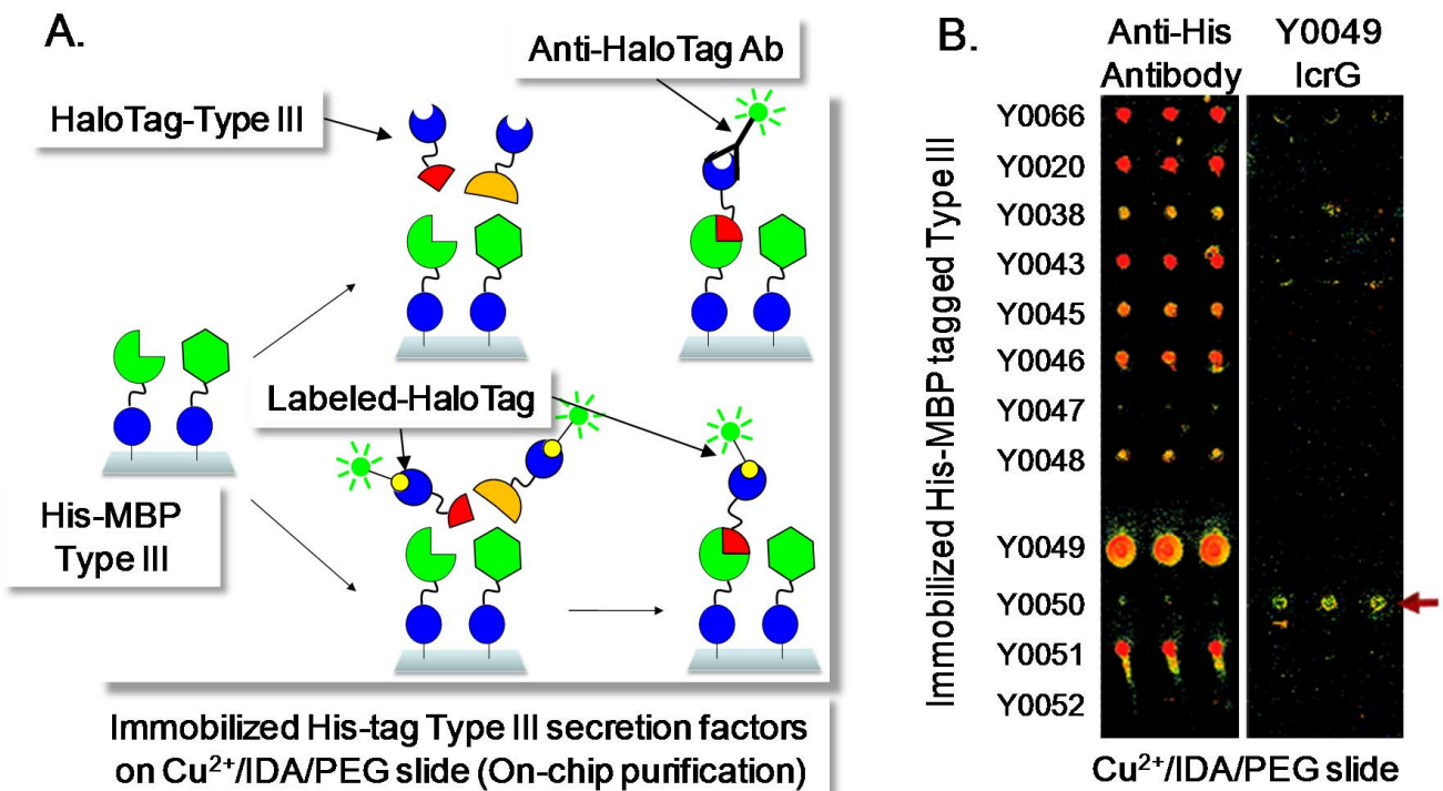
Fig. (4). Identification of T3SS Interactions in situ Using Protein Microarrays. (A) Scheme used to identify protein-protein interaction using HaloTag recombinant proteins and His-MBP tagged recombinant proteins. (B) Immobilized His-MBP tagged T3SSs on \text{Cu}^{2+} /IDA/PEG were visualized with anti-His-tag antibody (left) and interacting proteins with IcrG were detected by the rabbit anti-Halo antibody and goat anti-rabbit antibody labeled with Alexa555 (right).
