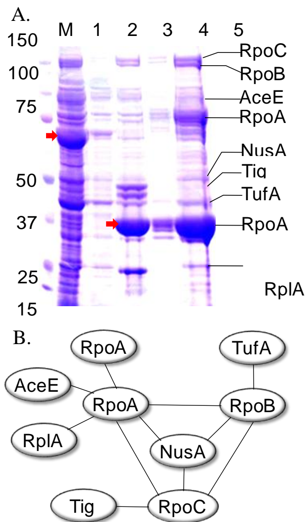
Fig. (5). Multi-protein Complex Discovery. (A) The pull-down study using HaloTag recombinant RpoA. M: molecular weight marker; 1: unbound protein; 2: wash; 3: eluted protein after TEV protease cleavage; 4: eluted protein after removal of TEV protease; 5: concentrated protein sample. The arrows indicate the position of HaloTag recombinant (lane 1) and cleaved (lane 3) RpoA. (B) Interaction map of E. coli proteins which identified by MALDI-MS/MS from the E. coli RpoA pull-down study.
