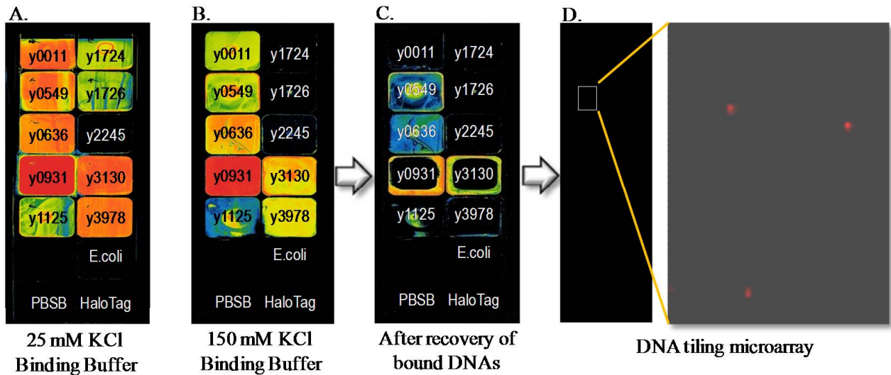
Fig. (6). Protein Microarray and DNA Tiling Microarray to Identify Protein-DNA Interactions. of hypothetical proteins in Y. pestis KIM. Binding of Cy5 labeled sheared genomic DNA onto a 16-pad protein array ( A ) in low salt binding buffer (25 mM KCl) and ( B ) in high salt buffer (150 mM KCl). ( C ) Array image after recovery of the bound DNAs. ( D ) DNA tiling microarray with the recovered DNA from protein array. The color represents the amount of DNA bound to the proteins. The color scale represents the strongest signals as red followed by orange, yellow, green, blue and black.
