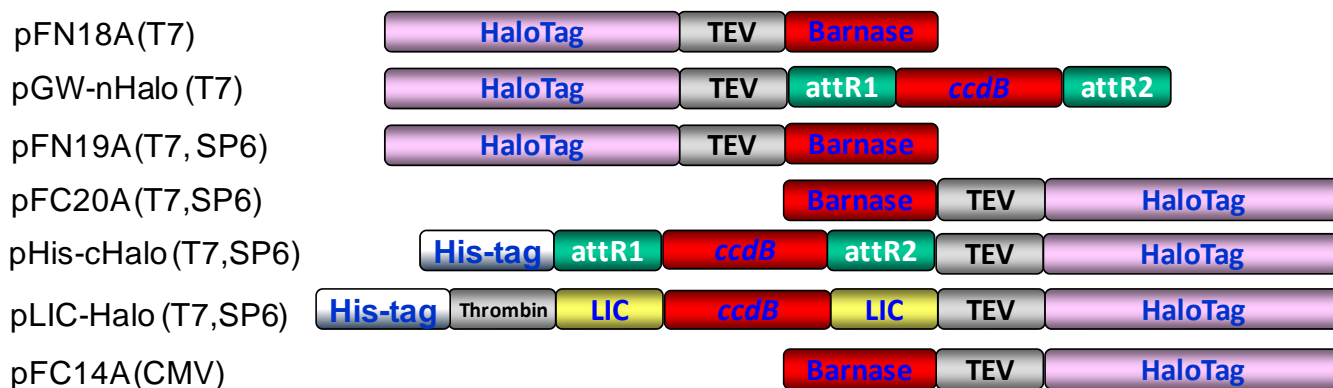
Fig. (1). The HaloTag expression vectors used for protein expression and functional studies.
