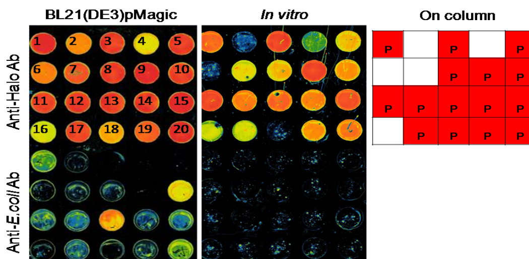
Fig. (3). A comparison of 20 proteins derived from S. pneumoniae using different expression and purification schemes. Manual in situ purification of E. coli , in vitro expressed proteins and column purification were compared. The purified proteins were visualized using rabbit anti-HaloTag antibody followed by a goat anti-rabbit antibody conjugated to the dye Alexa555 (upper). The purity of the proteins recovered from each strategy was examined by comparing the ratio of signal generated by an anti- E. coli antibody to that of anti-HaloTag antibody. Each well represents purification of the following protein, 1: SP_0291, 2: SP_0308, 3: SP_0321, 4: SP_0435, 5: SP_0604, 6: SP_0845, 7: SP_0954, 8: SP_0979, 9: SP_1102, 10: SP_1504, 11: SP_1572, 12: SP_1631, 13: SP_1650, 14: SP_1671, 15: SP_1699, 16: SP_1752, 17: SP_1802, 18: SP_1925, 19: SP_1959, and 20: SP_2209.
