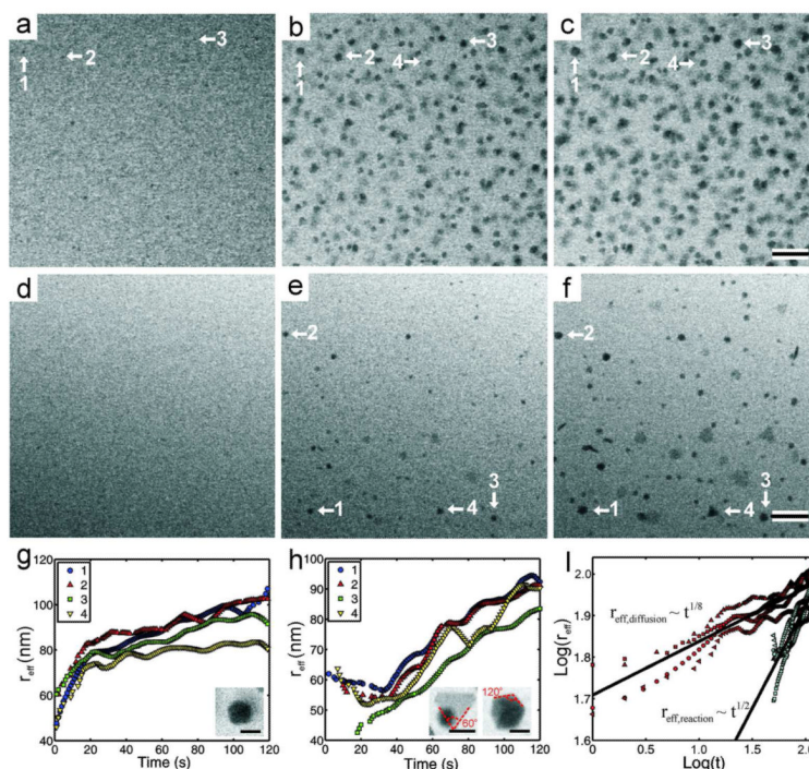
Figure 6. (a)-(c) Time series of BF-STEM images taken at t = 0 (a), 60 (b), and 120 s (c), with i_e = 40 pA, M = 100,000\times , 5 \mu\text{s} dwell time, resulting in an electron dose rate of 3.37 electrons/ (\text{\AA}^2\text{s}) . (d)-(f) Time series of BF-STEM images taken at t = 0 (d), 60 (e), and 120 s (f), with i_e = 7 pA, M = 100,000\times , 5 \mu\text{s} dwell time, resulting in an electron dose rate of 0.59 electrons/ (\text{\AA}^2\text{s}) . The scale bar for both time series is 200 nm. (g) Plot of the effective radius ( r_{\text{eff}} ) as a function of time for 4 individual nanocrystals indicated in (a)-(c) with arrows. Inset is a higher magnification image showing the near spherical morphology of the resulting nanocrystal, the scale bar is 100 nm. (h) Plot of the effective radius ( r_{\text{eff}} ) as a function of time for 4 individual nanocrystals indicated in (d)-(f) with arrows. Inset are higher magnification images showing the faceted morphology of the resulting nanocrystals, the scale bars are 100 nm. (i) Logarithmic relationship between the effective radius and time. The red data points correspond to (g) while the blue correspond to (h), the different markers correspond to the individual nanocrystals indicated in the legends of (g) and (h). The black lines are the average power law fits for the 4 different nanocrystals, obtained by linear regression. A 10 point averaging filter was used on (g), (h), and (i) to reduce noise in the data.
