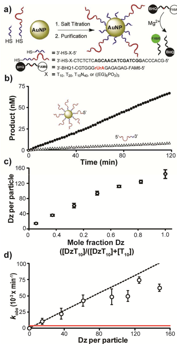
Figure 1. DzNP Synthesis and catalysis. (a) A schematic of the strategy used to generate DNAzyme gold nanoparticle conjugates (DzNPs). A binary mixture of two oligonucleotides, DNAzymes and passivating strands, were used to control the steric environment at the particle surface. The catalytic activity of DzNPs was determined by measuring the rate of fluorescence increase, which represents the rate of substrate hydrolysis and de-quenching. (b) A representative kinetic plot showing the rate of catalysis for 4.2 nM DzT 10 NP ([AuNP]=4.2nM) (closed circles) and DzT 10 (triangles) enzymes ([Mg 2+ ]= 50 mM). (c) A plot showing the DNAzyme surface density for T 10 passivated DzNPs as a function of the mole fraction of DNAzyme added during the NP functionalization. (d) A plot showing k_{\text{obs}} for the hydrolysis of a series of DzNPs that vary in DNAzyme surface density at [Mg 2+ ]= 10 mM. The horizontal red line denotes the activity of free DzT 10 (4.2 nM). The diagonal dashed line is a best fit ( R^2=0.99 ) through the lower density DzNP data points ( < 60 DNAzymes/particle). All error bars represent the standard deviation of three measurements.
