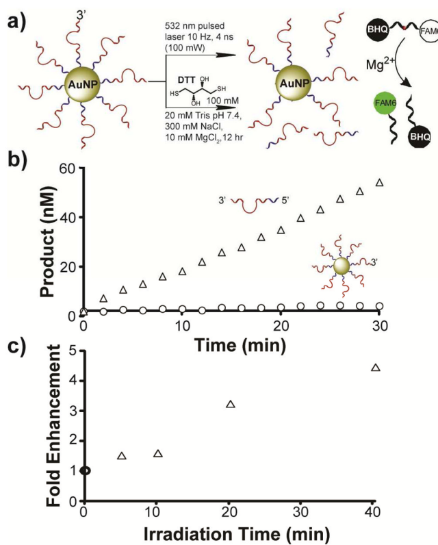
Figure 2. Triggering DNAzyme activity by partial release from particle surface. (a) Schematic showing DTT displacement (bottom) or laser irradiation (top) to release Dz rev T 10 from the particle to enhance catalysis. (b) A kinetic plot showing rate of catalysis of Dz rev T 10 NP (open circles) and DTT displaced Dz rev T 10 (open triangles) from the particle. (c) A plot showing k_{\text{obs}} as a function of irradiation time where the rate constant was normalized to particle at t = 0 min (open circle). Nd:YAG laser was operated at 10 Hz, 4 ns pulse width, generating 125 mW/cm 2 power.
