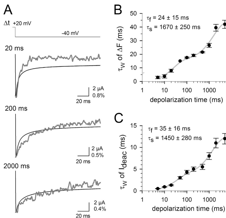
Figure 3. Direct correlation between VSD and gate movement in the Shaker -M356C channel using site-directed fluorimetry. (A) Simultaneous recording of I_{\text{deac}} (black traces) and recovery of fluorescence quenching ( \Delta F , gray traces) from an oocyte expressing TMRM-labeled M356C Shaker channels using the indicated protocol and various prepulse durations at 20 mV. For clarity, both traces have been normalized. The vertical scale bar indicates both ionic current amplitude (in microamps) and \Delta F/F (in percentage). (B) The kinetics of the fluorescence recovery signal obtained at -60 mV is shown as a function of the prepulse duration. Note that like the gating current recordings, there were two slowing processes in the kinetics with prolonged membrane depolarizations. (C) Development of the weighted I_{\text{deac}} time constant at -60 mV as a function of depolarization time, displaying, like the simultaneously recorded \Delta F signal, a biphasic slowing of the kinetics. Error bars represent SEM.
