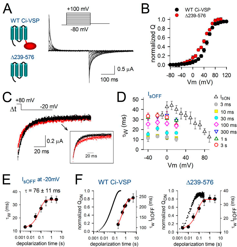
Figure 8. VSD relaxation in the isolated VSD of Ci-VSP. (A, left) Cartoon representation of the full-length WT Ci-VSP and the truncated mutant \Delta 239-576 that lacks the phosphatase domain (red) attached to the VSD (blue). (right) Sensing current traces ( I_s ) of the truncation mutant \Delta 239-576 recorded using the indicated activation protocol. (B) QV curves for the mutant \Delta 239-576 (red) and WT Ci-VSP (black) obtained by integrating the activating I_s from pulse protocols shown in A and Fig. 7 A, respectively. (C) A superposition of I_{sOFF} current traces at -20 mV after 10-ms (black) and 3-s (red) depolarizations to 80 mV is displayed. Note the slowing in I_{sOFF} decay and the reduction in the fast component amplitude of the red trace. The inset shows the normalized tracings to better highlight the slowing in I_{sOFF} decay. (D) Kinetics of activating I_{sON} (open triangles) of the mutant \Delta 239-576 obtained from different activation voltage pulses (similar to the protocol shown in A) and of deactivating I_{sOFF} of the same mutant obtained using 80-mV prepulses of the indicated durations from 3 ms to 3 s (colored symbols) and pulsing to different deactivation voltages. (E) Weighted time constant of I_{sOFF} decay measured at -20 mV as a function of the duration of the conditioning prepulse at 80 mV.
