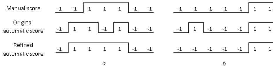
Fig. 2. Refinement of the automatic epoch score by a smoothing algorithm in two steps correcting the situations where: a) a single swallow is split into several parts by a misclassified epoch; b) accidental epochs are incorrectly classified as swallows
