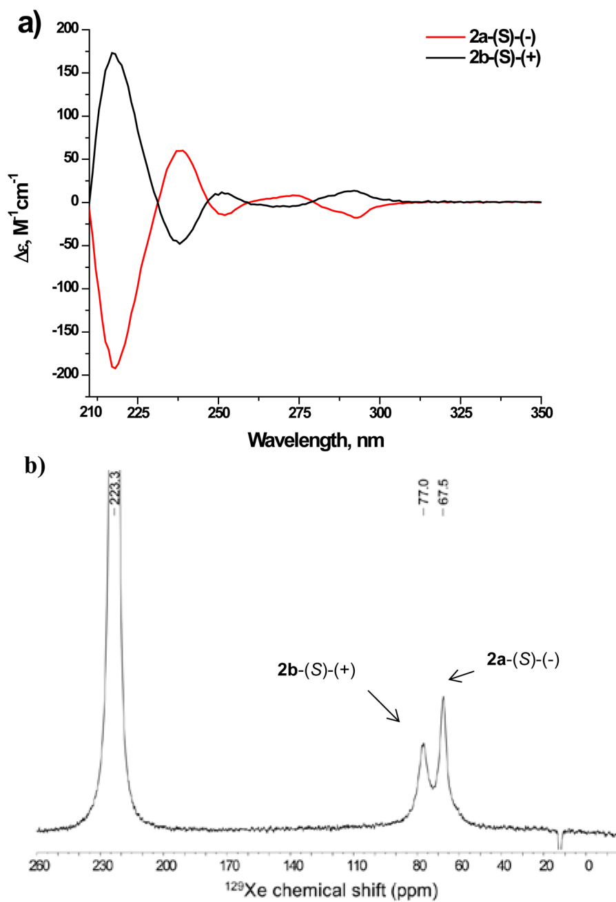
Figure 1. (a) ECD spectra of diastereomers 2a and 2b (~0.5 mM) in 1,4-dioxane. (b) Hyperpolarized ^{129}\text{Xe} NMR spectra of diastereomers 2a and 2b (~ 10 mM) in \text{C}_2\text{D}_2\text{Cl}_4 at 299 \pm 2 K.
