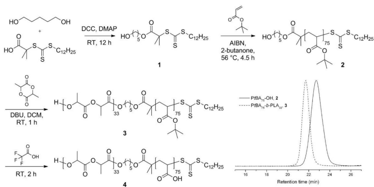
Figure 1. Synthetic scheme for the preparation of amphiphilic diblock copolymer PAA 75 - b -PLA 33 , 4 , and GPC traces of intermediates P t BA 75 -OH, 2 , and P t BA 75 - b -PLA 33 , 3 .
