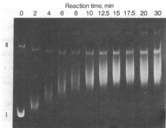
FIG. 5. BaP diol epoxide alkylation of SV40 DNA monitored by agarose gel electrophoresis. SV40 form I DNA ( 8.4 \mu\text{g}/\text{ml} ) reacted at 37^\circ\text{C} with BaP diol epoxide at a molar reaction ratio of 0.60. Samples ( 50 \mu\text{l} ) were taken at the indicated times and mixed with 10 \mu\text{l} of 2.5 M 2-mercaptoethanol to stop the reaction. The alkylated DNA was electrophoresed downward at 50 V for 12 hr on a 1.4% agarose slab gel. The decrease in mobility and broadening of the form I DNA band are attributed to local unwinding of the helix by BaP diol epoxide adducts and to strand scission during the electrophoretic analysis.
