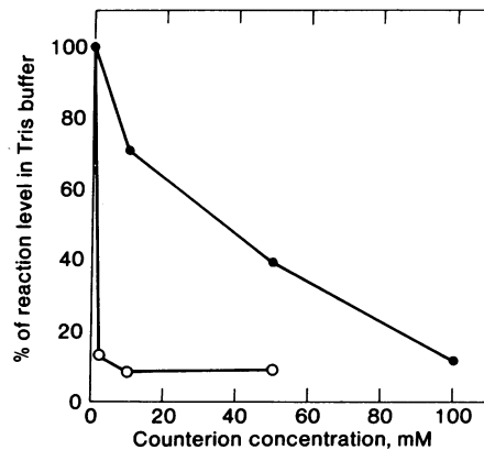
FIG. 2. Inhibition of BaP diol epoxide alkylation of SV40 DNA by NaCl and MgCl 2 . SV40 form I [ 14 C]DNA reacted with [ 3 H]BaP diol epoxide at a molar reaction ratio of 0.60 in the presence of the indicated concentrations of NaCl (●) or MgCl 2 (○). The DNA control contained 197 adducts per genome.
