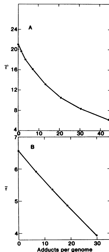
FIG. 4. Removal of superhelical turns by BaP diol epoxide adducts in superhelical (A) and partially relaxed (B) SV40 DNA.
