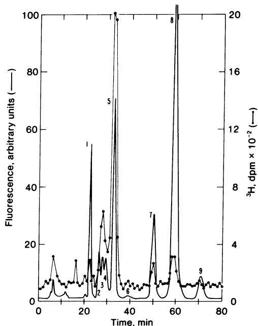
FIG. 1. High-pressure liquid chromatography profile of co-injection of [ 3 H]BaP diol epoxide-SV40 DNA adducts plus unlabeled BaP diol epoxide-calf thymus DNA adducts. The form I viral DNA was allowed to react with [ 3 H]BaP diol epoxide at a molar reaction ratio of 0.04. Peaks 3, 5, and 6 are deoxyguanosine adducts; peaks 7, 8, and 9 are deoxyadenosine adducts; and peaks 2 and 4 are deoxycytidine adducts. Peak 1 and part of peak 4 consist of 7,8,9,10-tetrahydroxy-7,8,9,10-tetrahydrobenzo[ a ]pyrene. The two early eluting radioactive peaks probably represent BaP diol epoxide solvent-addition products. Counting efficiency was 38%.
