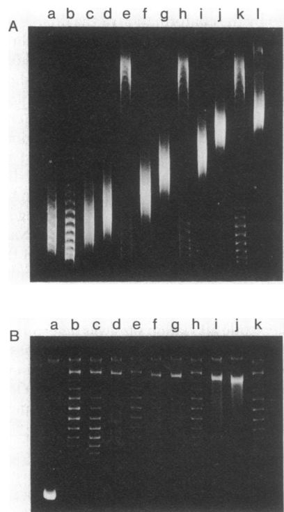
FIG. 3. (A) Polyacrylamide slab gel of superhelical SV40 DNA that had reacted with BaP diol epoxide. SV40 form I [ ^{14}\text{C} ]DNA reacted for 90 min at 37°C with [ ^3\text{H} ]BaP diol epoxide at molar reaction ratios of: a, 0.002; b, 0; c, 0.005; d, 0.01; f, 0.02; g, 0.04; i, 0.06; j, 0.10; and l, 0.15. Samples were electrophoresed downward for 72 hr at 100 V on a 2% polyacrylamide/0.5% agarose slab gel. Tracks e, h, and k contained partially relaxed form I SV40 DNA. The top band in each track is form II SV40 DNA. (B) Agarose slab gel of partially relaxed SV40 DNA that had reacted with BaP diol epoxide. Partially relaxed SV40 form I [ ^{14}\text{C} ]DNA reacted with [ ^3\text{H} ]BaP diol epoxide at molar reaction ratios of: c, 0; d, 0.02; f, 0.04; g, 0.06; i, 0.10; and j, 0.15. After 3 hr at 37°C, samples were electrophoresed downward for 16 hr at 50 V on a 1.4% agarose slab gel. Tracks b, e, h, and k contained a mixture of SV40 DNAs incubated for 15 min or for 20 min with DNA-relaxing enzyme. Track a contained superhelical DNA. The top band in each track is unresolved low molecular weight cellular DNA; the second band is form II viral DNA.
