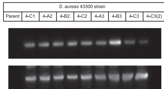
FIG 5 Western blot assays of S. aureus ATCC 43300 and its AFN-1252-insensitive derivatives. Top panel shows detection of FabI and bottom panel shows FtsZ.
