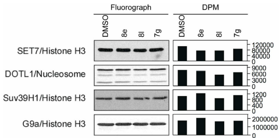
Figure 4. Inhibitory activities of 7g , 8e , and 8l against a panel of HKMTs (SET7, DOTL1, Suv39H1, and G9a) using the indicated histone and/or non-histone substrates.
