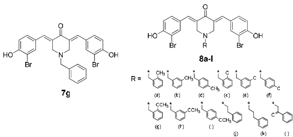
Figure 1. CARM1-selective inhibitors used in this study.
