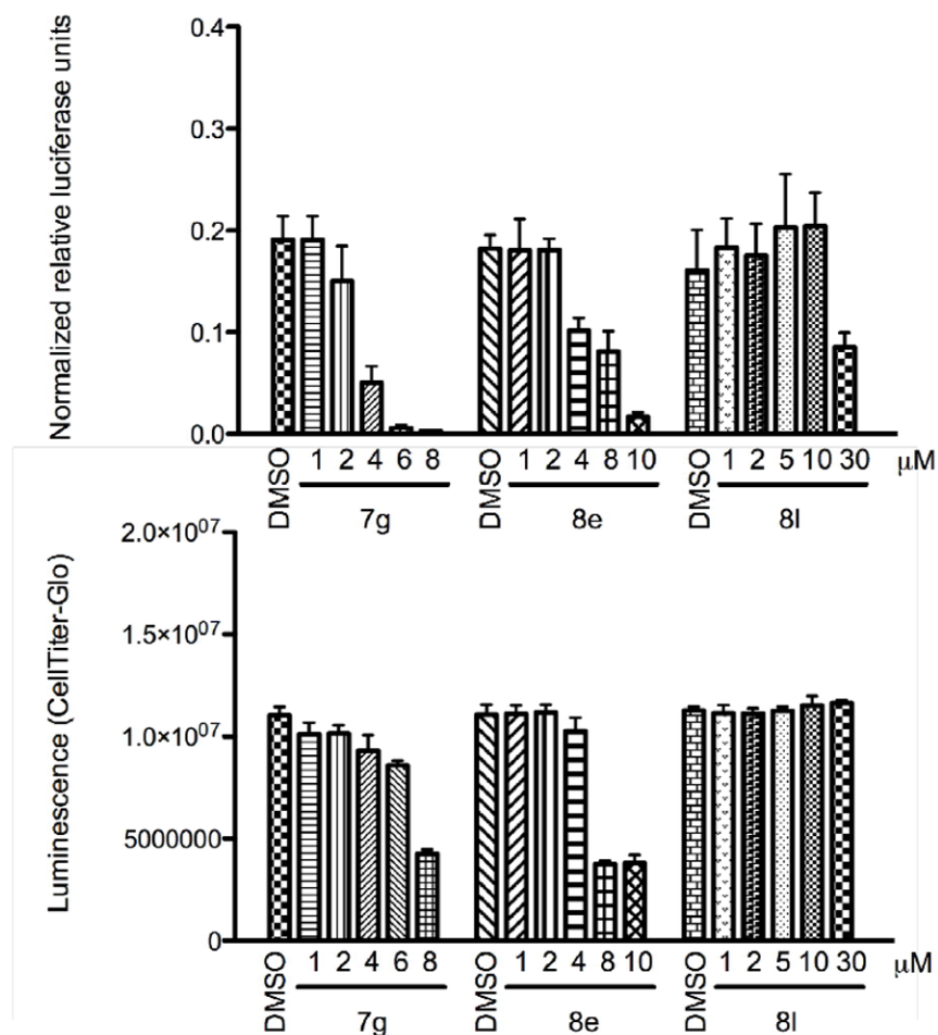
Figure 5. Effects of increasing concentrations of 7g , 8e , and 8l on PSA promoter activity by luciferase assay in LNCaP cells, relative to a CMV-Renilla control (top panel), and on cell viability based on quantitation of the ATP present, which is an indicator of metabolically active cells, and is used to determine the viability of cells in culture (bottom panel). The results are presented as mean \pm SD that were calculated from triplicate luciferase assays.
