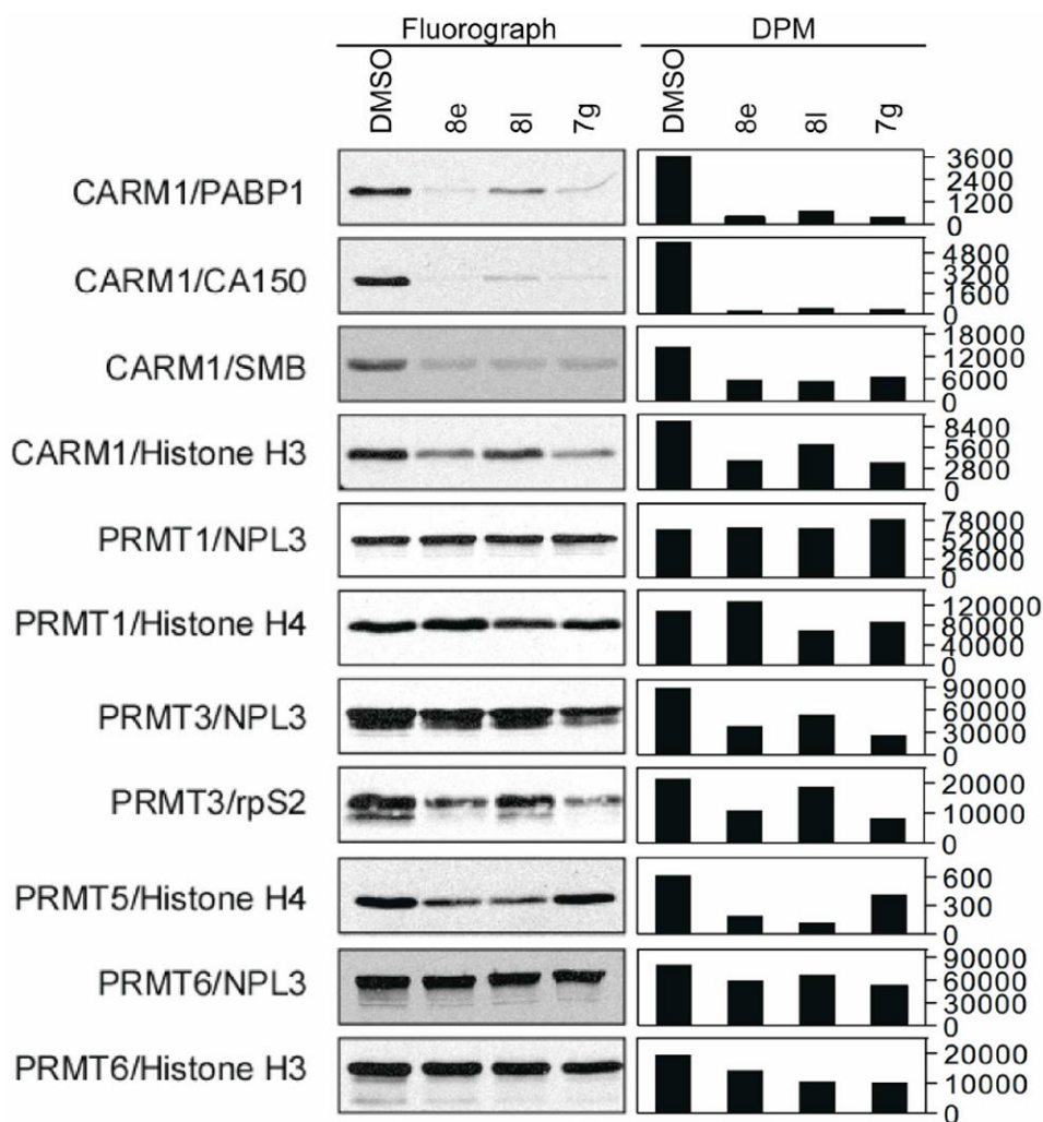
Figure 3. Inhibitory activity of 7g , 8e , and 8l against CARM1 using PABP1, CA150, SMB, and histone H3 as substrates, and against a panel of PRMTs (PRMT1, PRMT3, PRMT5, and PRMT6) using indicated histone and/or non-histone substrates. The fluorographs are shown in the left panels, and the tritium count for each band is depicted in the right panels.
