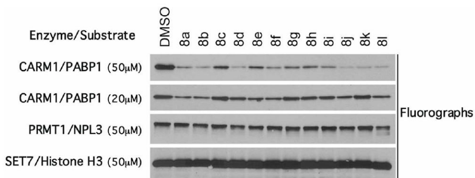
Figure 2. Inhibitory activities of compounds 8a-1 against CARM1 using PABP1 as a substrate, PRMT1 using NPL3 as a substrate, and SET7 using histone H3 as a substrate. The concentration of the compounds used in each in vitro methylation assay is shown.
