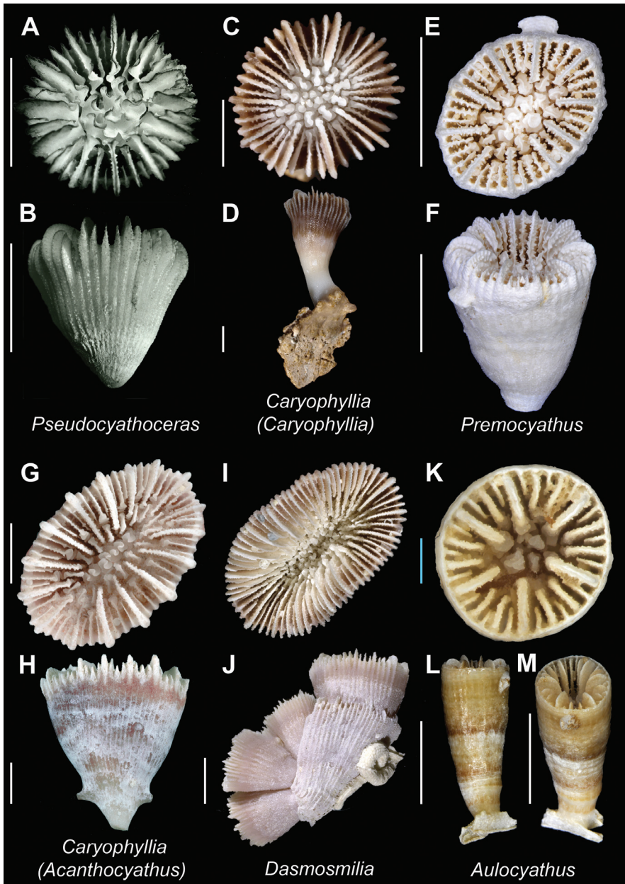
Plate 16. Pseudocyathoceras avis (USNM 46962, holotype) A and B Calicular and lateral view respectively; Caryophyllia (Caryophyllia) quadragenaria (USNM uncatalogued, PrFO, New Caledonia) C and D Calicular and oblique view respectively; Premocyathus dentiformis (MNHN uncatalogued, Ebisco stn. DW2573) E and F Calicular and oblique view respectively; Caryophyllia (Acanthocyathus) grayi (MNHN uncatalogued, Ebisco stn. DW2559) G and H Calicular and lateral view respectively; Dasmosmilia lymani (USNM 82997) I and J Calicular and lateral (aggregation) view respectively; Aulocyathus juvenescens (MNHN uncatalogued, Lifou 2000 stn. DW37) K , L , and M Calicular, lateral, and oblique view respectively. Scale bars: blue = 1 mm; white = 5 mm. Bold face indicates type species for the genus.
