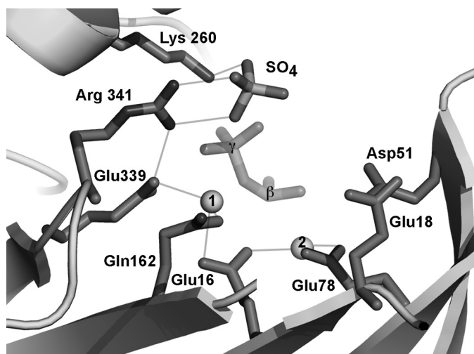
FIGURE 6. Synthetic representation of the three-dimensional structure of the VgrG1 ACD active site residues, cation-conserved sulfate anion, and the \beta - and \gamma -phosphates of ATP.
