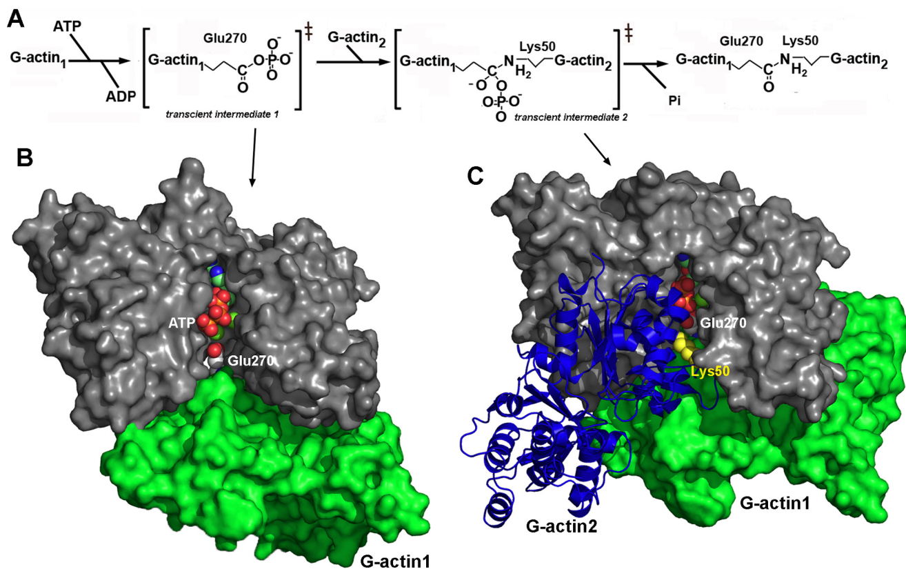
FIGURE 4. The catalytic mechanism catalyzed by VgrG1-ACD. A, schematic representation of the two-step mechanism (adapted from Satchell (8)). B, model of the first transient intermediate of VgrG1-ACD with G-actin1. G-actin 1 Glu-270 is close enough to the ATP \gamma -phosphate for transfer. C, model of the second transient intermediate of VgrG1-ACD with G-actin 1 and G-actin 2. G-actin 2 Lys-50 is in favorable position for nucleophilic attack on phosphorylated Glu-270 to occur, leading to a covalent amide bond between Glu-270 and Lys-50 side chains.
