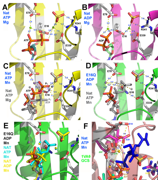
FIGURE 5. Three-dimensional structure of the VgrG1 ACD active site. A, native complex with ATP and Mg^{2+} . B, native complex with ADP and Mg^{2+} . C, native complex with ATP and Mn^{2+} compared with the complex with ATP and Mg^{2+} (gray sticks). D, E16Q variant complex with ADP and Mn^{2+} compared with the native complex with ATP and Mn^{2+} (gray sticks). E, E16Q variant complex with ADP and Mn^{2+} compared with the native complex with ATP and Mn^{2+} (blue sticks) and with the native complex with ADP and Mn^{2+} (yellow sticks). F, native VgrG1 ACD complex with ATP and Mn^{2+} (sticks) compared with the superposed structure of GCS (Protein Data Bank code 1VA6; side chains colored by atom type with violet carbons) in complex with ADP (green), Mg^{2+} (violet spheres), and the phosphosulfoximine inhibitor (blue sticks). The labels of the pairs of corresponding residues have identical colors, but GCS labels are italicized.
