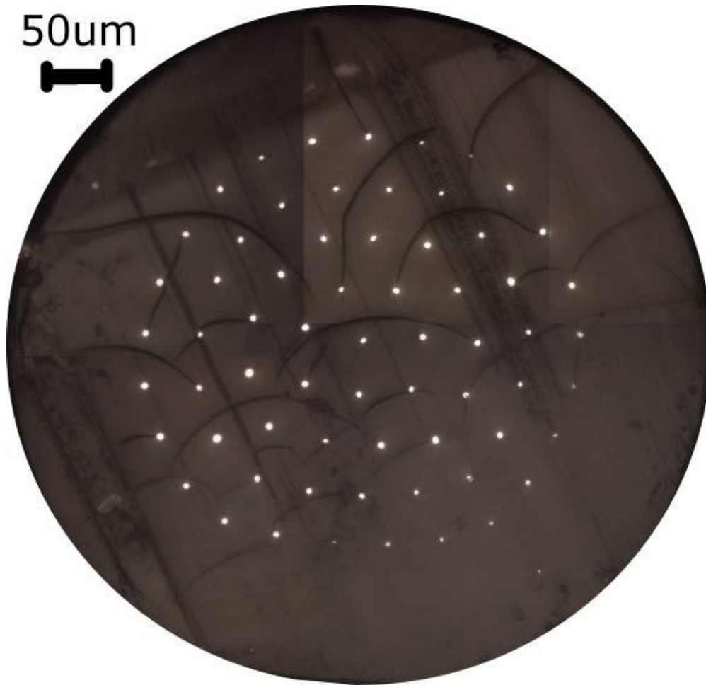
Figure 3. (Composite) optical microscope cross sectional image of the 5 \mu\text{m} indium wires separated by 50 \mu\text{m} in a PMMA fiber. (40x objective lens).
