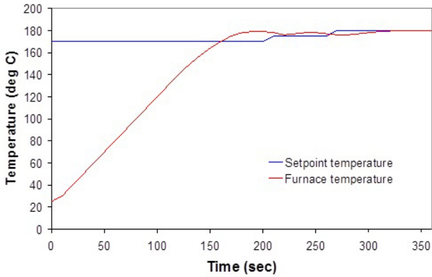
Figure 14. Pre-heat profile.
