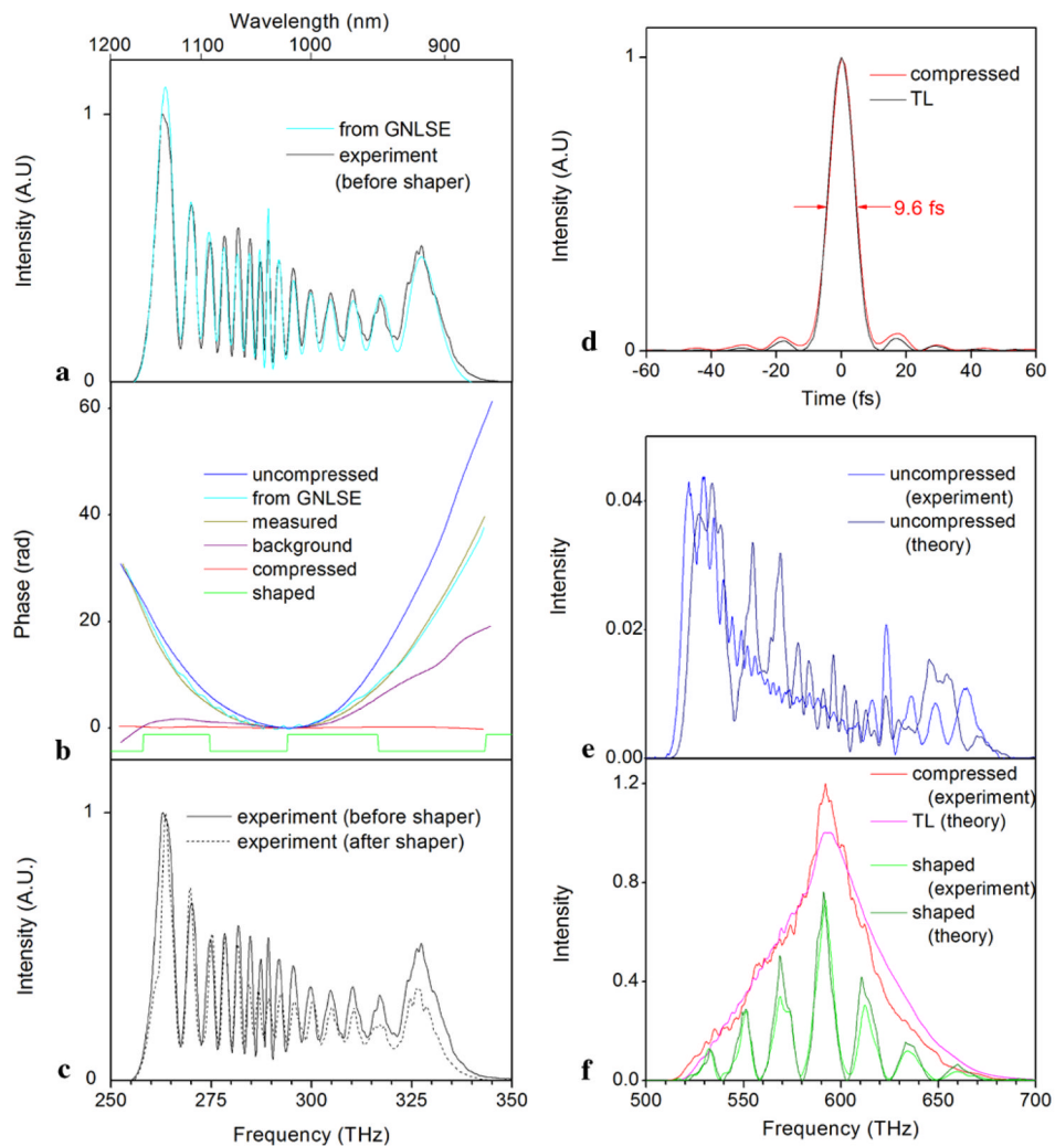
Fig. 2. (a) Measured spectrum of fiber continuum source and the scalar GNLSE-quantified spectrum. (b) Comparison of the spectral phases corresponding to the uncompressed pulses, the scalar GNLSE-quantified fiber continuum pulses, the measured pulses, the background of the MIIPS-integrated pulse shaper, the compressed pulses, and the shaped pulses (see details in text). (c) Comparison of measured spectrum of fiber continuum source (before shaper) and measured spectrum of fiber continuum at the focus of the curved mirror (after shaper). (d) Reconstructed temporal profiles of the compressed pulses and the corresponding TL pulses. (e) Comparison of the measured and calculated SHG spectra of the uncompressed pulses. (f) Comparison of the measured SHG spectrum of the compressed pulses and the calculated SHG spectrum of the TL pulses, and of the measured and calculated SHG spectra of the shaped pulses
