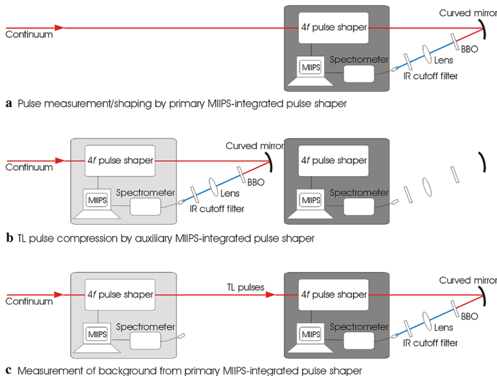
Fig. 1. Scheme for absolute pulse measurement by MIIPS. The background of the pulse measurement by the primary MIIPS-integrated pulse shaper ( a ) is obtained by the pulse compression in ( b ) and the subsequent measurement in ( c ) with the assistance of an auxiliary MIIPS-integrated pulse shaper
