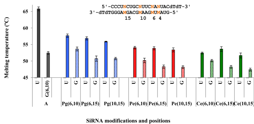
Figure 5. Thermal analysis of siRNA duplexes with double 8-alkoxyA modifications at three different positions, 6, 10 and 15, in the guide strand. Modifications were placed opposite to U or G in the corresponding passenger strands. The sequences are shown in the Figure 2; here X is 8-PgOA, 8-PeOA or 8-CeOA, and N is either U or G.
