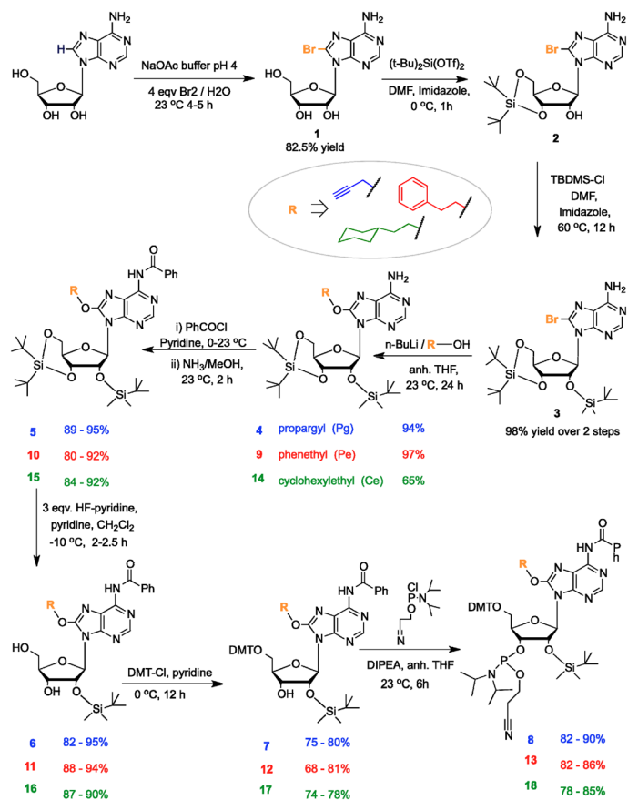
Figure 2. Synthesis of the 8-alkoxyadenosine phosphoramidites.
