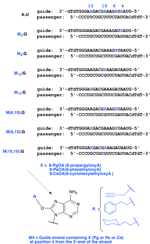
Figure 3. SiRNA sequences used. A:U represents unmodified siRNA and modified (denoted by M:G) sequences have the standard A:U base pair replaced by 8-alkoxy(X):G in one or two positions in the siRNAs.
