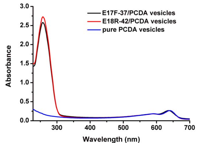
Figure 2. UV-vis absorbance spectra of pure PCDA vesicles before (blue curve) and after binding aptamers (red and black curve).
