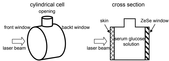
Fig. 3. Schematic diagram of sample holder
