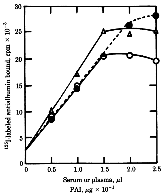
FIG. 2. Immunoreactivity of a PAI preparation (albumin-IgG complexes) (●), fresh and untreated human serum (Δ), and plasma (○) treated first with monospecific anti-IgG and then with ^{125}I -labeled antialbumin.
