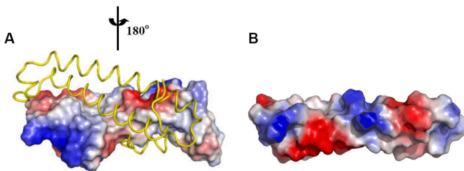
Figure 10. Surface potentials of TraM At (PDB ID: 1RFY) and TraM NGR (PDB ID: 2Q0O) (from the anti-activation complex). For dimeric TraM At , surface of one monomer is shown, the other monomer is shown as a C \alpha trace in yellow. Surface with positive potentials is colored in blue, and with negative potentials in red. TraM NGR is shown in the same view as the surface presentation of TraM At monomer.
