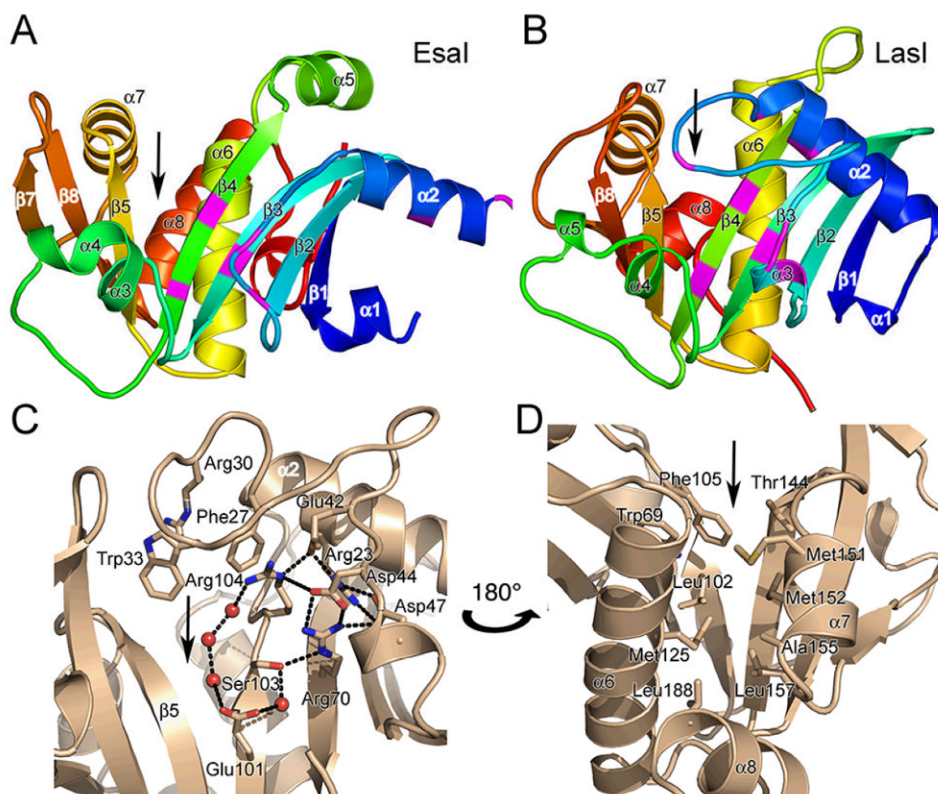
Figure 5. Structure of the AHL synthases EsaI and LasI. (A) Ribbon diagrams depict the backbone structures of EsaI (A) and LasI (B). The structure of the EsaI enzyme (PDB ID 1kzf) from Pantoea stewartii was determined from the native sequence. The structure of the LasI enzyme (PDB ID 1ro5) from Pseudomonas aeruginosa was determined from an active form that had been engineered to improve solubility and crystallization properties. The rainbow coloring is blue to red from the N-terminus to the C-terminus and the major secondary structure elements are labeled. The most conserved residues are indicated with magenta coloring. (C) Close-up view of the LasI active site residues, showing the conserved residues and the electrostatic cluster. Well-ordered water molecules in the active site are shown as red spheres and putative hydrogen bonds are shown as dotted black lines. (D) Close-up view of the LasI acyl-chain binding pocket. The view is rotated approximately 180° about the vertical axis of the page relative to (C) and shows the residues lining the putative acyl-chain binding pocket. In each panel, the active site V-shaped cleft is indicated with a black arrow.
