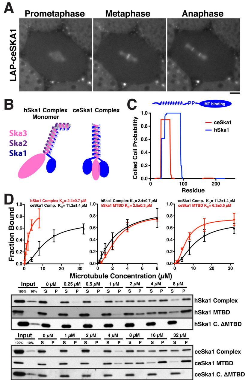
Figure 1. The C-terminus of Ska1 is the conserved microtubule-binding domain of the Ska1 complex
