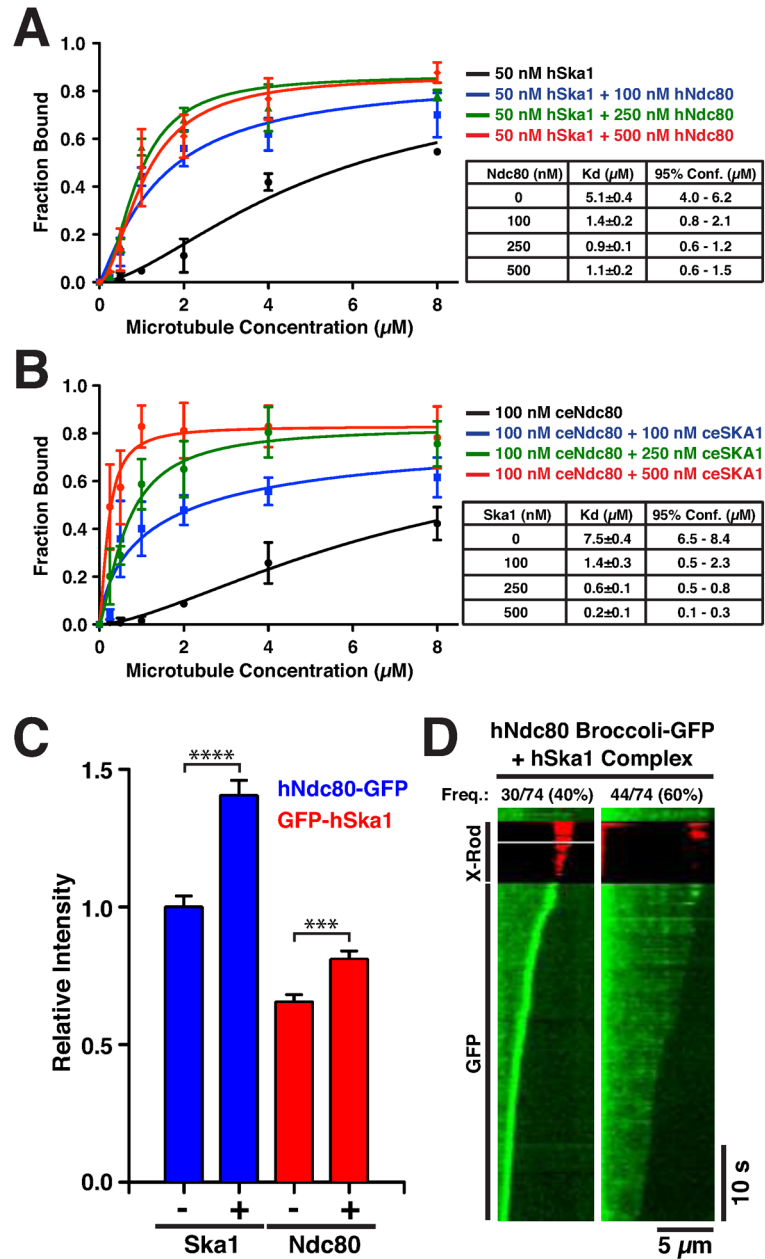
Figure 6. The Ska1 complex confers microtubule tracking activity to the Ndc80 complex (A) The Ska1 complex and Ndc80 complex bind to microtubules synergistically. Quantification of microtubule co-sedimentation assays for hSka1 complex binding to taxol-stabilized microtubules alone and in the presence of a range of concentration of hNdc80 “Broccoli” (Mean \pm SD, n = 3). (B) Quantification of microtubule pelleting assays of C. elegans Ndc80 complex binding to taxol-stabilized microtubules alone and in the presence of a range of ceSKA1 complex (n = 3). (C) Quantification of the fluorescence intensity (Mean \pm SEM) on microtubules of hNdc80 “Broccoli”-GFP (blue) in the absence (n = 95) and presence of hSka1 (n = 136; P < 0.0001, t-test), and GFP-hSka1 (red) in the absence (n = 73) and presence of hNdc80 “Broccoli” (n = 81; P < 0.001, t-test). (D) Representative kymographs (microtubule position along horizontal axis, time along vertical axis) of time-lapse movies showing hNdc80 “Broccoli”-GFP (9 nM) binding to depolymerizing
