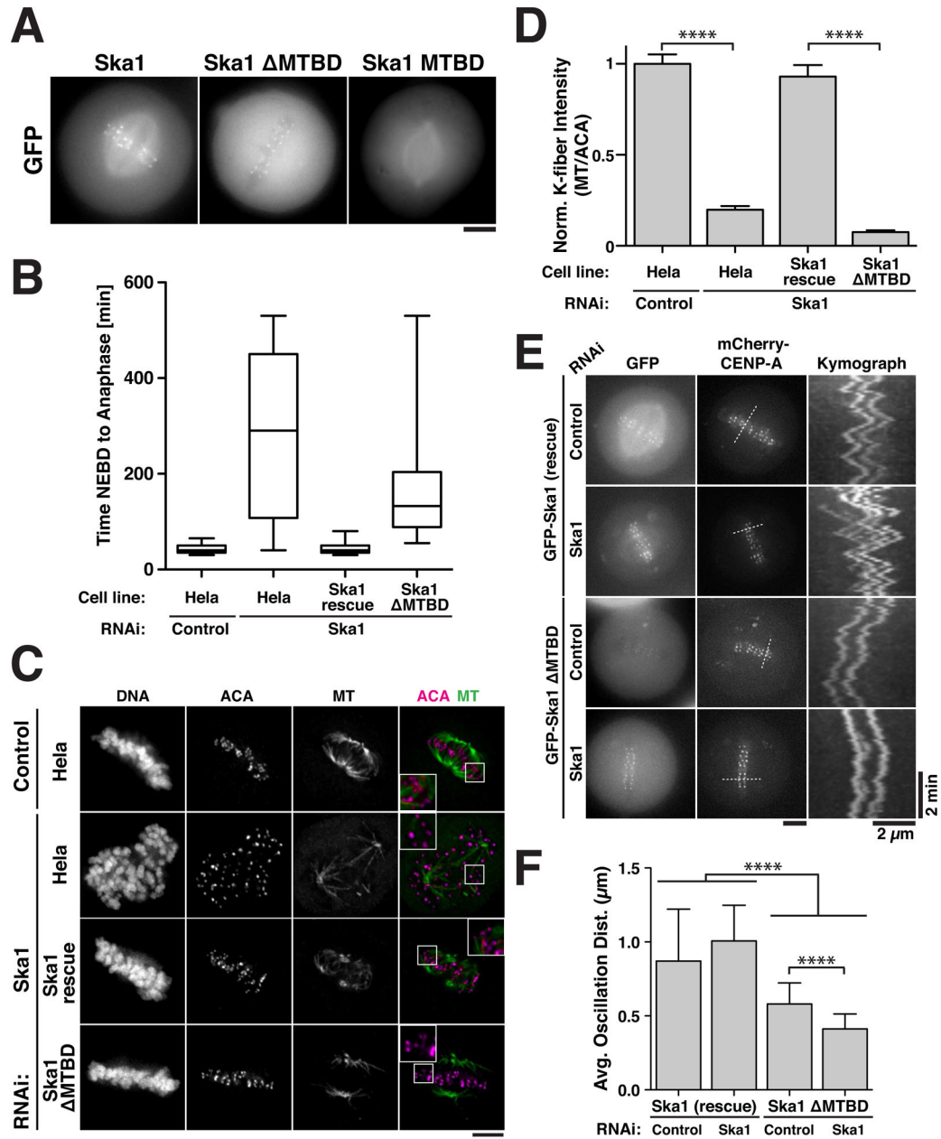
Figure 2. The microtubule-binding activity of the Ska1 complex is required for mitotic progression and kinetochore-microtubule attachments
