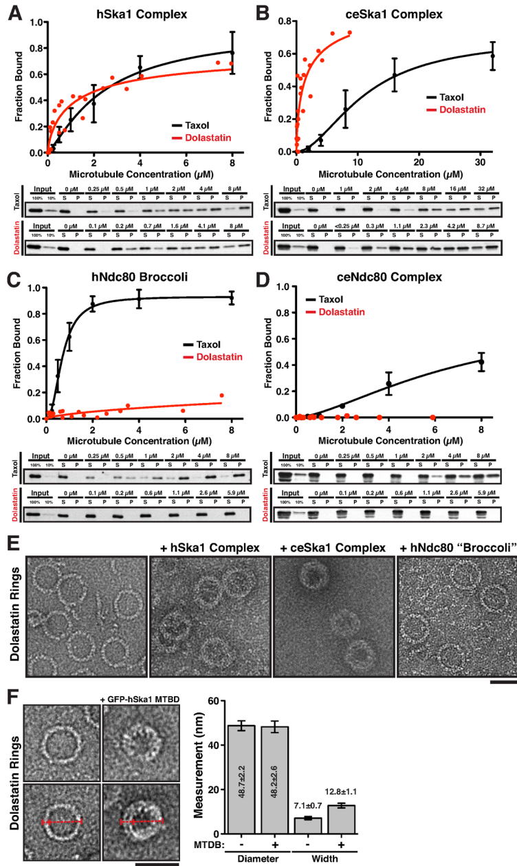
Figure 5. The Ska1 complex, but not the Ndc80 complex, associates with depolymerizing microtubule end mimics (A–D) (Top) Quantification of microtubule co-sedimentation assays (Mean \pm SD, n = 3) and (Bottom) representative Western blots of microtubule co-sedimentation assays of (A) hSka1 complex (100 nM, 75 mM KCl), (B) ceSka1 complex (100 nM, 75 mM KCl), (C) hNdc80 “Broccoli” (100 nM, 75 mM KCl), and (D) ceNdc80 complex (100 nM, 75 mM KCl) binding to taxol stabilized microtubules (black) and dolestatin-10 induced protofilament rings (red). (E) Transmission electron microscopy (TEM) images of dolestatin-10 induced protofilament rings alone or decorated with the ceSka1 complex or hSka1 complex, and in the presence of hNdc80 “Broccoli” (Scale bars, 40 nm). (F) Left, TEM images showing individual dolestatin-10 rings in the presence or absence of the GFP-hSka1 microtubule-binding domain (MTBD; Scale bar, 50 nm). Right, graph showing the outer diameter and
