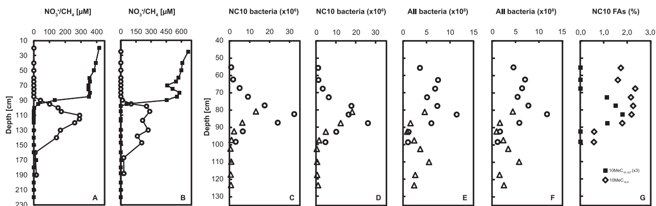
FIG 1 Depth profiles of the Brunssummerheide peatland. (A and B) Nitrate (filled square) and methane (open circle) concentrations in porewater sampled in December 2009 (A) and in June 2010 (B). (C to F) Bacterial cell numbers (cells \text{g}^{-1} wet soil) as assessed by qPCR on DNA extracted from two overlapping soil cores from 51 to 102 cm (open circles) and from 77 to 127 cm (open triangles). NC10 bacterial abundance was determined with primer pairs p1F and p1R (C) and p2F and p2R (D). Total bacterial abundance was determined with primer pair 535F and 805R (E) and 1100F and 1492R (F). (G) Relative abundance of the fatty acids 10-methyl-hexadecanoic acid (10MeC 16:0 ; open diamonds) and 10-methyl-hexadec-7-enoic acid (10MeC 16:1 Δ 7 ; multiplied by 3; closed squares), which are diagnostic of NC10 bacteria (data are from Kool et al. [24a]).
