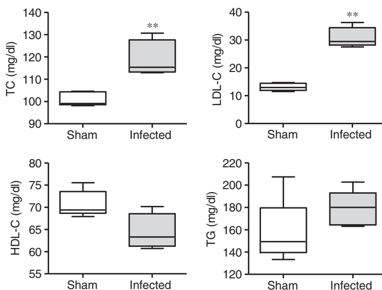
Figure 2 Effects of P. gingivalis infection on the plasma lipid profile (N = 5 in each group). Box plots represent medians, with the 25 th and 75 th percentiles as boxes and the 10 th and 90 th percentiles as whiskers. Total and LDL cholesterol levels were significantly higher, whereas HDL cholesterol levels tended to be lower in the P. gingivalis -infected mice (** P < 0.01 , Mann-Whitney U-test).
