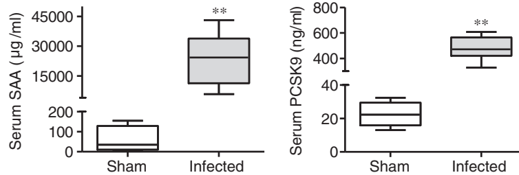
Figure 1 Effects of P. gingivalis infection on serum levels of serum amyloid A (SAA) and PCSK9 (N = 5 in the sham-infected group; N = 6 in the infected group). All samples were analyzed in duplicate for each condition. Box plots represent medians, with the 25 th and 75 th percentiles shown as boxes and the 10 th and 90 th percentiles as whiskers. Significant differences were observed between the infected group and the sham-infected group (** P < 0.01 , Mann-Whitney U-test).
