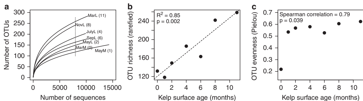
Figure 2 Successional changes in bacterial diversity. (a) The rarefaction curves show the observed 97% OTU richness with increasing sequencing depth of the kelp biofilm sampled across a gradient of kelp surface age (March 2007–November 2007, see Supplementary Figure S1). Sample id is indicated by abbreviated month names and ‘L’ and ‘M’ for the kelp lamina and meristem, respectively. Numbers in parentheses indicate the approximate age of the kelp surface in months. The dotted line shows at what sequencing depth rarefied OTU richness was calculated. (b) Rarefied 97% OTU richness increases with kelp surface age. (c) 97% OTU evenness, measured by Pielou’s evenness index, increases with kelp surface age.
