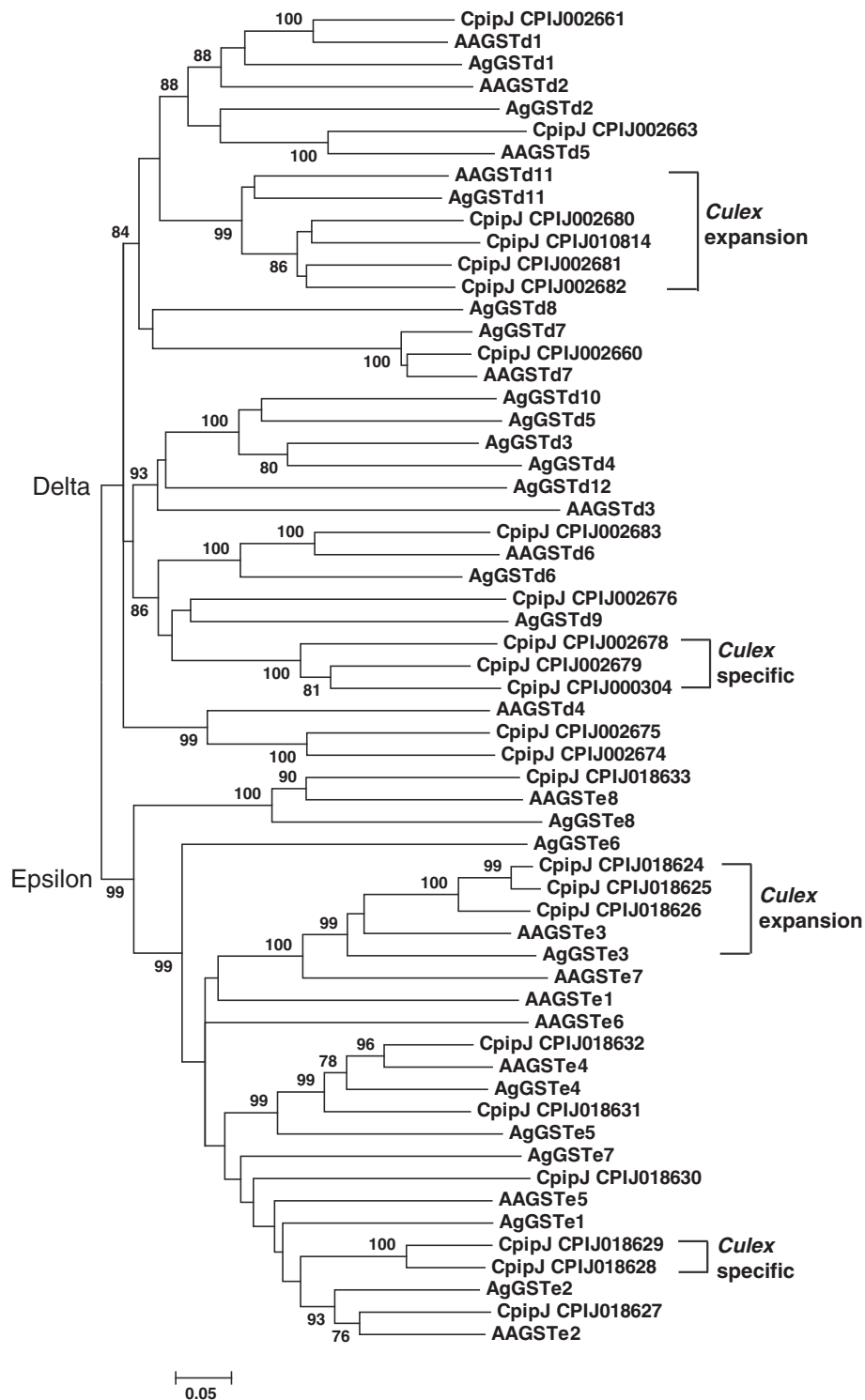
Figure 7 Unrooted distance neighbor-joining tree showing the phylogeny of delta and epsilon glutathione S-transferases from the genome of Culex pipiens quinquefasciatus in relation to those from Aedes aegypti (initiated with 'AA') and Anopheles gambiae (initiated with 'Ag'). The percentage of bootstrap confidence values greater than 70% (1000 replicates) is shown at the nodes.
