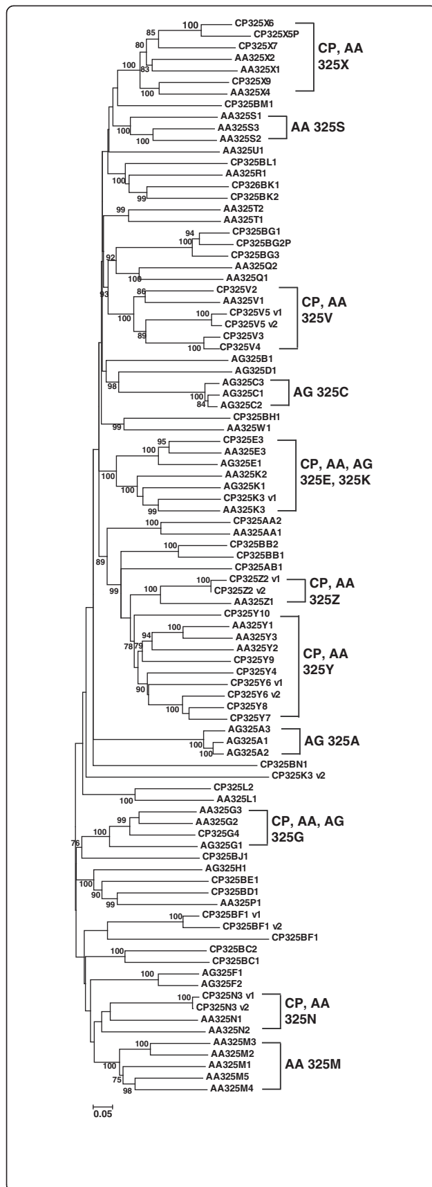
Figure 5 Unrooted distance neighbor-joining tree showing the phylogeny of P450 CYP325 genes from the genome of Culex pipiens quinquefasciatus (initiated with 'CP') in relation to those from Aedes aegypti (initiated with 'AA') and Anopheles gambiae (initiated with 'AG'). The percentage of bootstrap confidence values greater than 70% (1000 replicates) is shown at the nodes.
