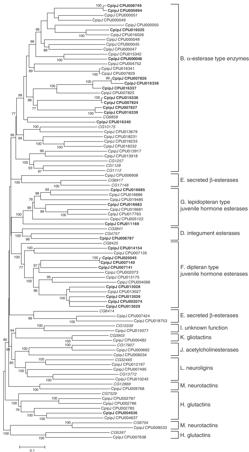
Figure 1 Unrooted distance neighbor-joining tree showing the phylogeny of carboxyl/cholinesterases (CCEs) from the genome of Culex pipiens quinquefasciatus in relation to CCEs from Drosophila melanogaster (in italics). CCEs of C. p. quinquefasciatus undetected in DGE libraries are shown in bold. The percentage of bootstrap confidence values greater than 70% (1000 replicates) is shown at the nodes. The functional assignment of clades follows the new system proposed by Oakeshott et al. [9].
