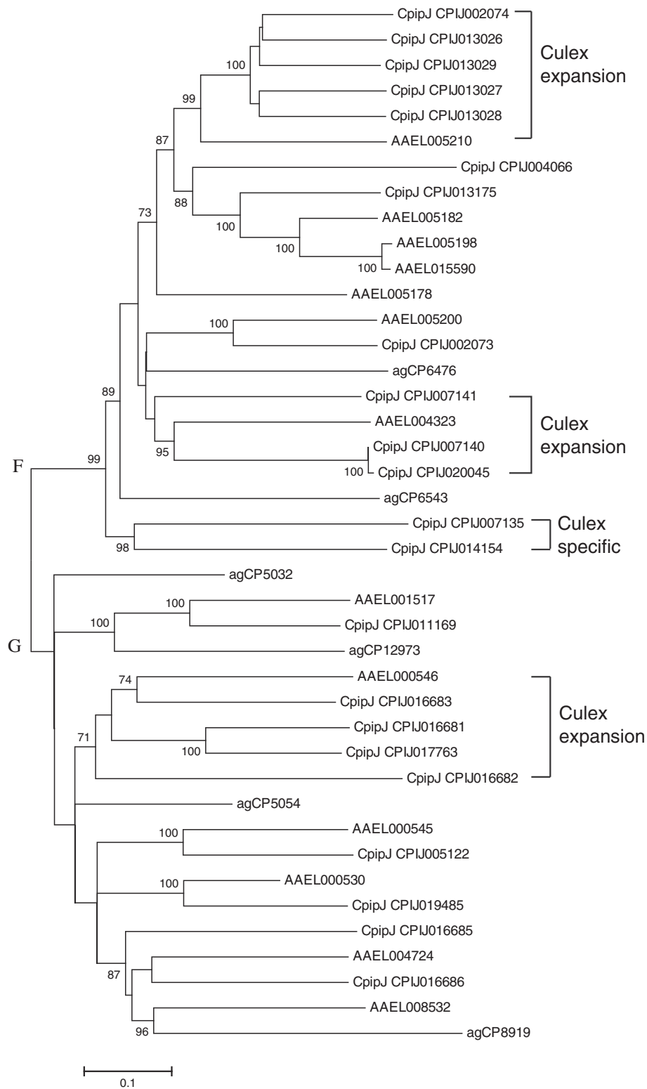
Figure 3 Unrooted distance neighbor-joining tree showing the phylogeny of juvenile hormone esterases from the genome of Culex pipiens quinquefasciatus in relation to those from Aedes aegypti (initiated with 'AAEL') and Anopheles gambiae (initiated with 'agCP'). The percentage of bootstrap confidence values greater than 70% (1000 replicates) is shown at the nodes.
