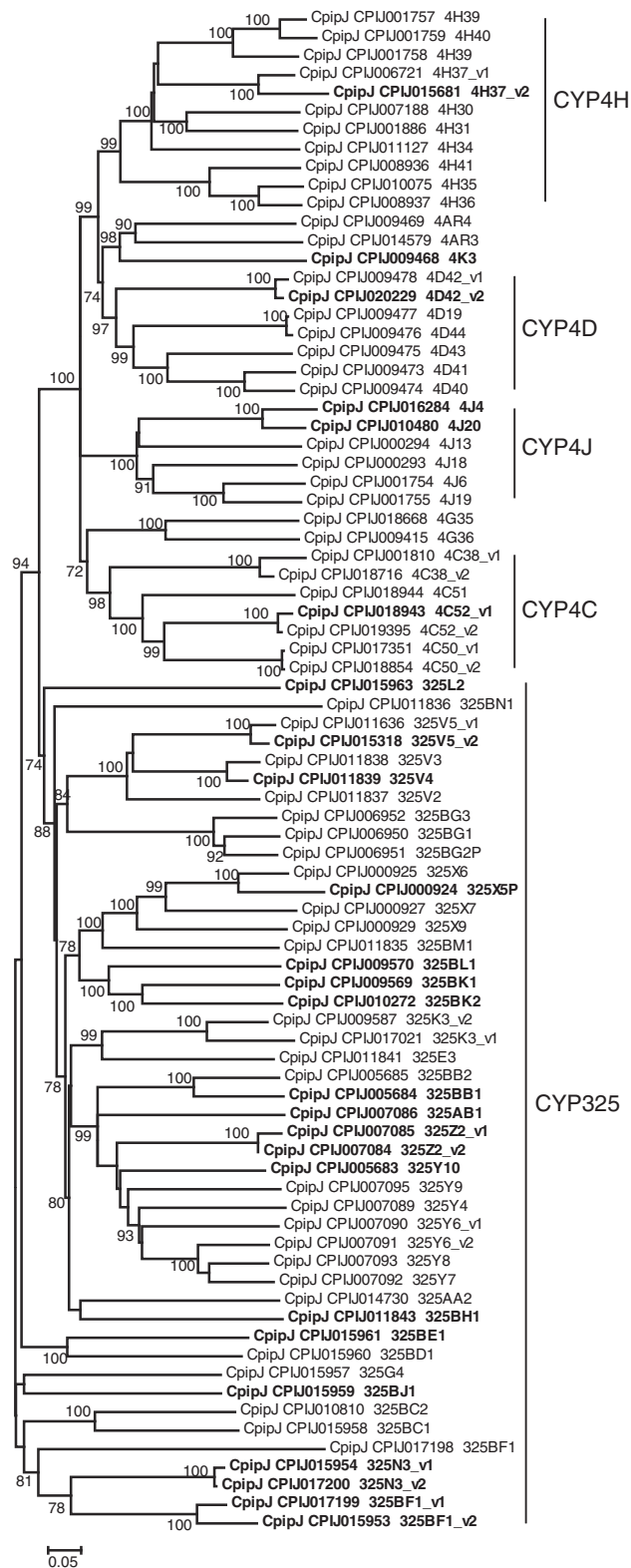
Figure 4 Unrooted distance neighbor-joining tree of P450 CYP4 genes from the genome of Culex pipiens quinquefasciatus . Greater than 70% support in 1000 bootstrap replications is indicated at the corresponding nodes. Genes undetected in DGE libraries are shown in bold. P450s were named by the P450 nomenclature committee ( http://drnelson.uthsc.edu/CytochromeP450.html ). Genes with v1 and v2 designation are very recent duplications and have not yet been assigned individual gene names.
