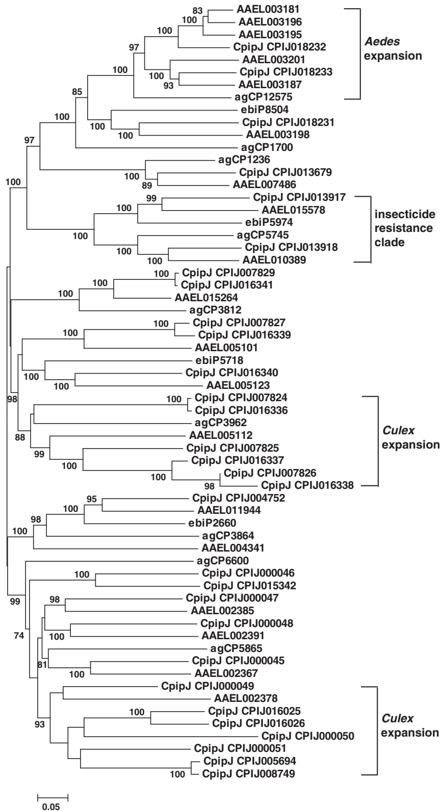
Figure 2 Unrooted distance neighbor-joining tree showing the phylogeny of \alpha -esterases from the genome of Culex pipiens quinquefasciatus in relation to those from Aedes aegypti (initiated with 'AAEL') and Anopheles gambiae (initiated with 'agCP' or 'ebiP'). The percentage of bootstrap confidence values greater than 70% (1000 replicates) is shown at the nodes.
