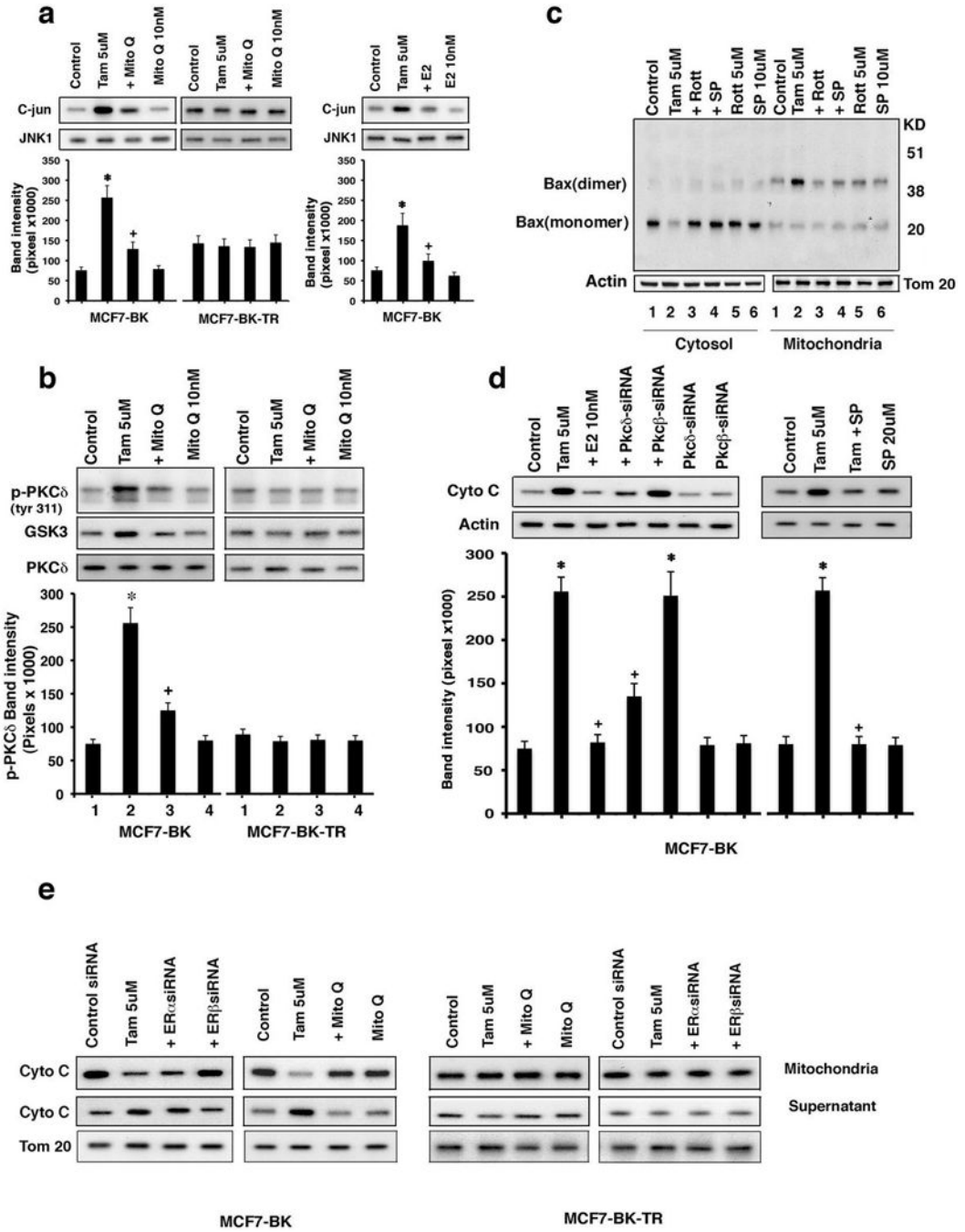
Figure 6. TAM activates JNK and PKC \delta in MCF7-BK to induce apoptosis (a) JNK activity or (b) PKC \delta kinase assays in cells exposed to TAM \pm Mito-Q or E2. Total protein was used as a normalization factor. Bar graphs are JNK activity or PKC \delta tyr311 phosphorylation from 3 expts. * p < 0.05 for TAM; + p < 0.05 for TAM versus TAM + Mito Q or TAM + E2. (c) Bax translocation to mitochondria and dimerization induced by TAM in BK cells but not to TAM \pm Rottlerin (PKC \delta inhibitor) or SP600125 (JNK inhibitor). The study was repeated. (d) TAM causes cytochrome C release via PKC \delta or JNK into BK cell cytosol. Bar graph is 3
