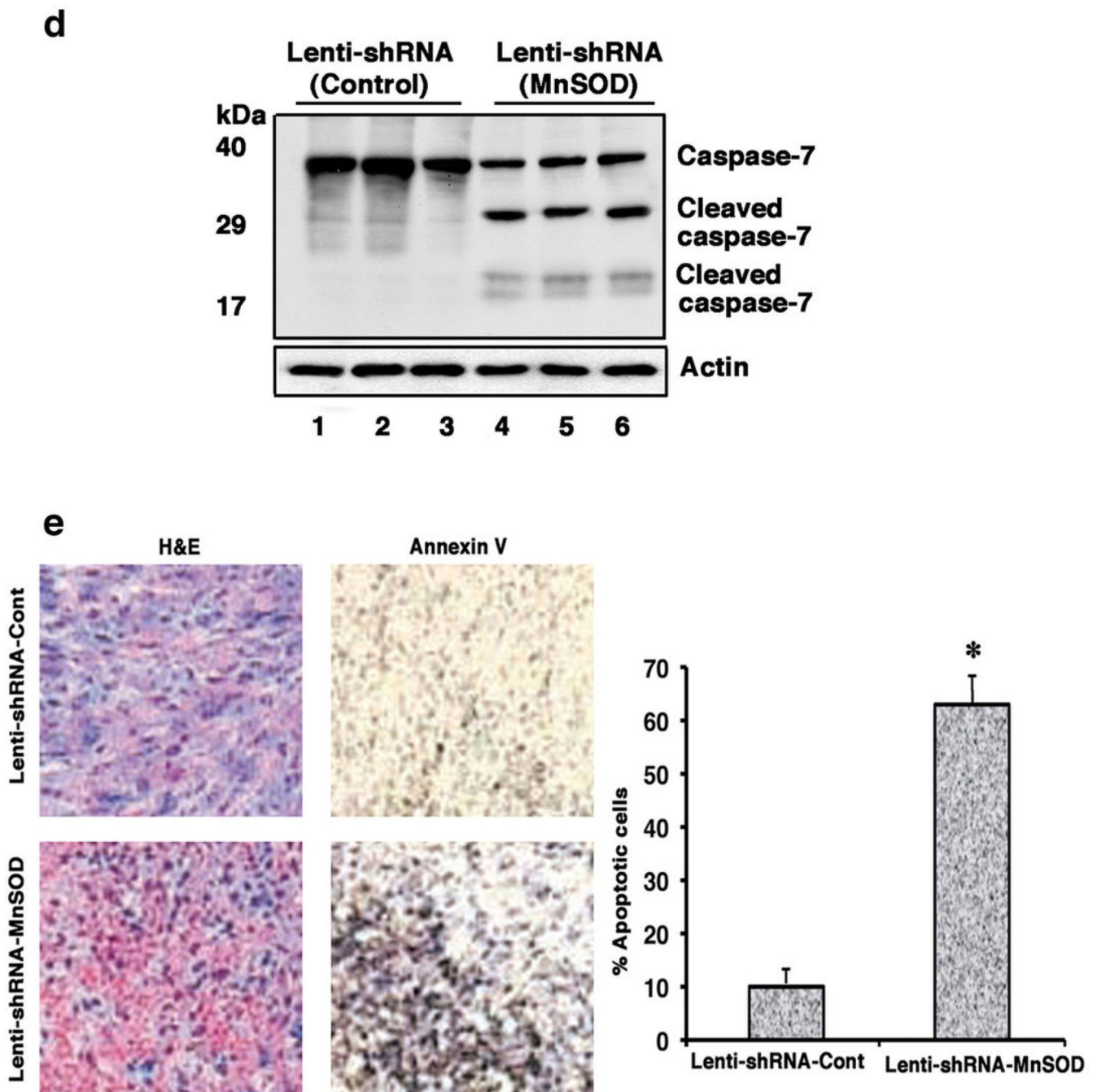
Figure 7. MnSOD knockdown disrupts the in-vivo growth of TAM resistant breast tumors (a), Left, MnSOD knockdown restores sensitivity to the tumor-repressing effects of TAM. Pictures are representative in-vivo tumors from 3 mice. Arrows indicate the tumors. Right, line graphs of measured in-vivo tumor volumes (n=6 mice). *p<0.05 for control versus MnSOD lenti-viral shRNA injected tumors. (b), Ex-vivo tumor volumes (n=6) (left) and pictures of extracted tumors from 3 mice. *p<0.05 for tumors injected with control shRNA versus MnSOD shRNA. (c) MnSOD protein immuno-blot from 3 tumors in each group. Actin is
