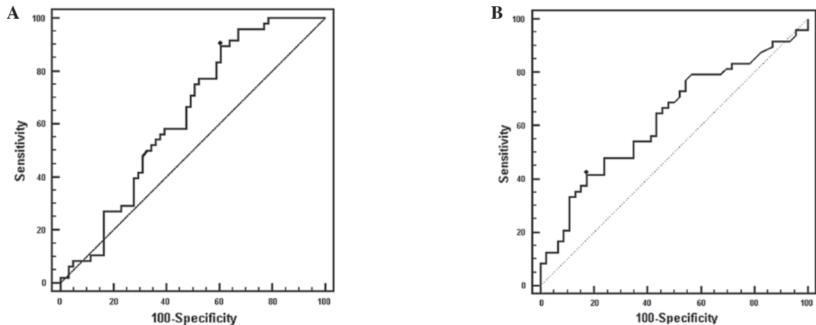
Figure 3. ROC curves: Early HCC. (A) ROC curve showing sensitivity and specificity of sCD25 in the detection of early stage HCC. The cut-off value of 2,859 pg/ml for sCD25 had a sensitivity of 89.6% and a specificity of 39.3% (AUC=0.630). (B) At a cut-off value of 20.6 ng/ml AFP possessed a sensitivity of 41.7% and specificity of 82.6% (AUC=0.630). sCD25 demonstrated a stronger capacity to predict early cancer (P<0.0001) than AFP (P=0.0257). ROC, receiver operator characteristic; HCC, hepatocellular carcinoma; sCD25 soluble CD25; AUC, area under the ROC curve; AFP, α-fetoprotein.
