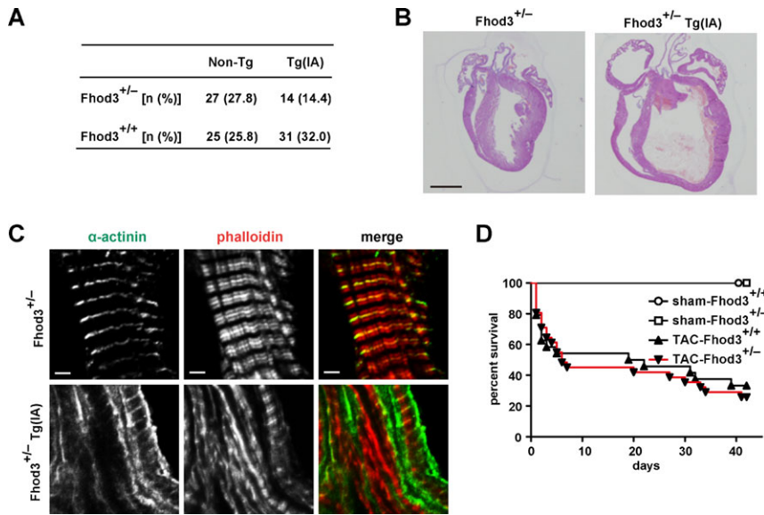
Fig. 5. Transgenic expression of Fhod3 (H1127A) in the heart. (A) Genotypes of offspring from the mating of Fhod3 +/- × Fhod3 +/- Tg( \alpha -MHC-Fhod31A). The number in parentheses indicates the percentage of the total number of offspring. (B) Histological analysis of hearts from Fhod3 +/- and Fhod3 +/- Tg( \alpha -MHC-Fhod31A) ( Fhod3 +/- Tg(IA)) mice at age 8 day. Bars, 100 \mu m. (C) Confocal fluorescence micrographs of hearts from Fhod3 +/- and Fhod3 +/- Tg( \alpha -MHC-Fhod31A) ( Fhod3 +/- Tg(IA)) mice at P8. Sections of hearts were subjected to immunofluorescent staining for \alpha -actinin (green) and phalloidin staining for F-actin (red). Bars, 2 \mu m. (D) Kaplan-Meier survival curves versus days after TAC. TAC- Fhod3 +/+ ( n=24 ); TAC- Fhod3 +/- ( n=31 ); sham- Fhod3 +/+ ( n=4 ); and sham- Fhod3 +/- ( n=4 ) mice.
