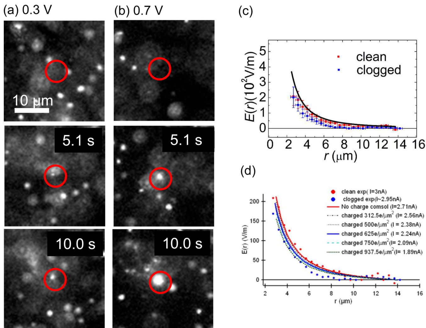
Figure 6. Fluorescence images showing the DNA clogging into a nanopore with bias voltage 0.3 V for (a) and 0.7 V for (b). Images are extracted at 5.1 sec and 10.0 sec after the first DNA molecule is clogged. A nanopore is located at the center of a drawn red circle in the images. One and three DNA molecules were clogging while two and five molecules entered nanopore at 5.1 sec and 10.0 sec for (a). Near 10 and 20 DNA molecules are clogged by 5.1 sec and 10.0 sec for (b). (c) The magnitude of the electric fields near the clean nanopore and DNA clogged nanopore on the nanopore membrane surface. The magnitudes of the fields are reduced for the DNA clogged pore. (d) Computer simulation shows that a charged nanopore surface can reduce the electric field near a nanopore.
