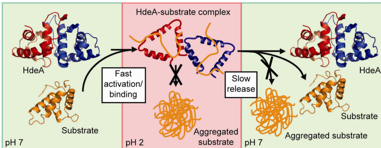
Figure 3. Mechanism of action of the flexible protein HdeA. At neutral pH (pH 7, left panel), HdeA exists as an inactive dimer. When exposed to acid (pH 2, center panel), HdeA, like many other proteins, unfolds and becomes more flexible. Although this unfolding process inactivates most other proteins, it triggers the activation of HdeA. The flexibility of HdeA allows it to mold itself to fit other proteins that have become aggregation-prone by acid-induced unfolding, thereby preventing their aggregation. HdeA slowly releases proteins after shifting to neutral pH (pH 7, right panel), keeping the concentration of aggregation-sensitive folding intermediates low.
