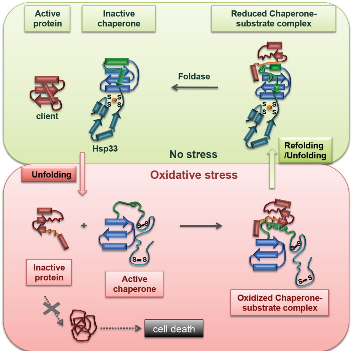
Figure 4. Mechanism of Hsp33, a redox-regulated chaperone. Under non-stress conditions, Hsp33 is a chaperone-inactive, zinc-binding monomer (upper left). Upon exposure to oxidative stress conditions that cause protein unfolding (e.g., bleach stress, oxidative heat stress), Hsp33 undergoes massive conformational rearrangements, triggered by the formation of two intramolecular disulfide bonds and zinc release (orange ball). This leads to unfolding of the C-terminal redox switch domain (cyan and green), and the activation of Hsp33 as chaperone (dimerization of Hsp33 has been omitted for simplicity). The linker region (green) of Hsp33 appears to directly interact with secondary structure elements of newly unfolded client proteins (red), adopting a more stabilized conformation in this process (lower right). Return
