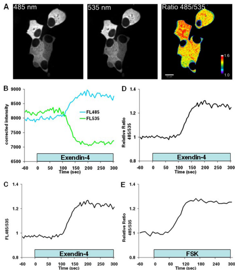
Fig. 1. cAMP biosensor expression and function in MIN6 cells
