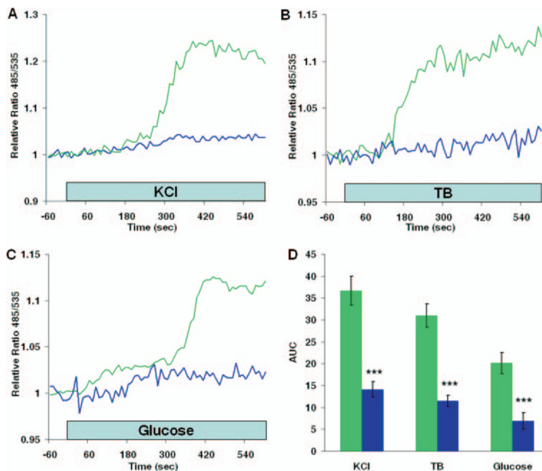
Fig. 2. Effect of secretagogues on cAMP formation
