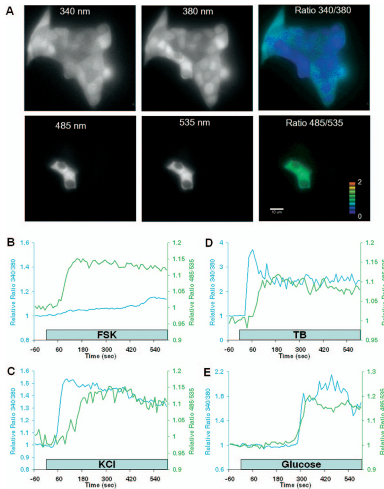
Fig. 4. Simultaneous imaging of cytoplasmic \text{Ca}^{2+} and cAMP signaling
