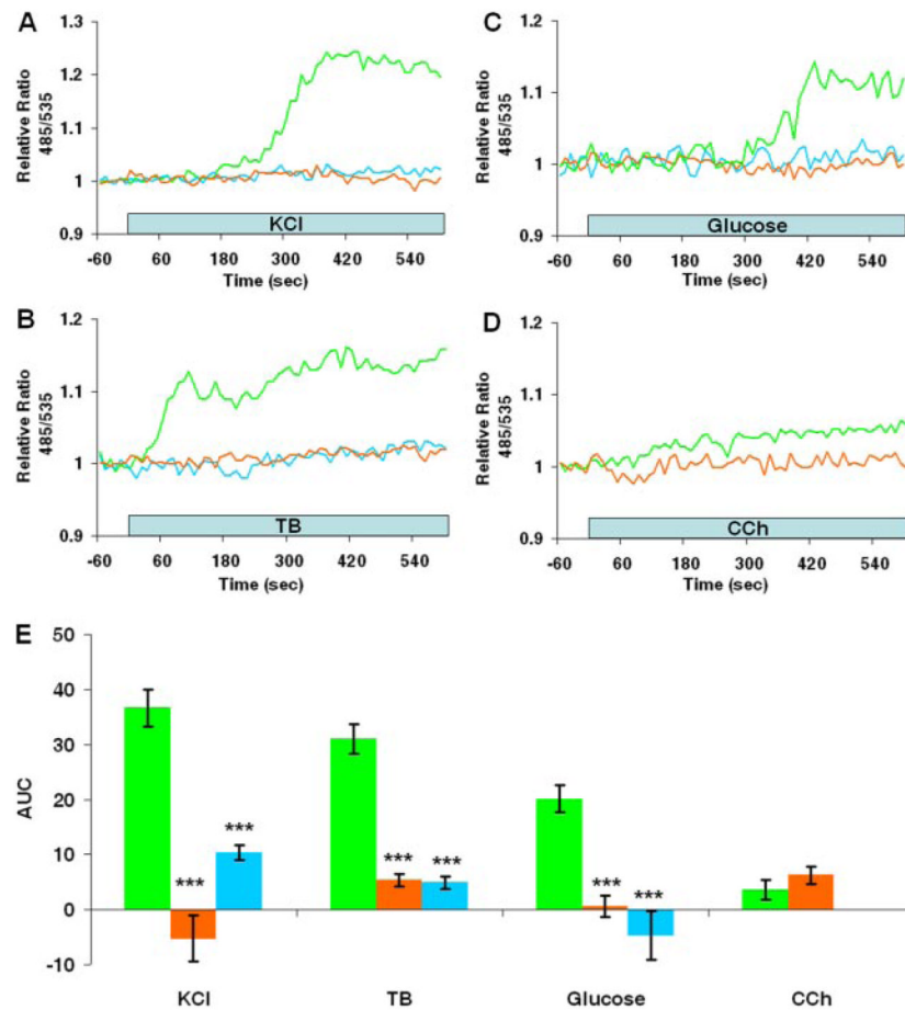
Fig. 3. Ca 2+ -dependent cAMP production in MIN6 cells
