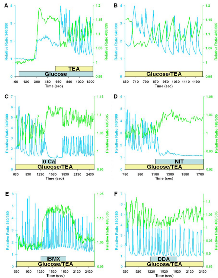
Fig. 5. Intracellular Ca^{2+} and cAMP oscillations
