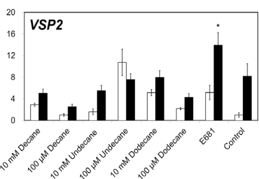
Figure 4. Induced resistance and priming of defense-related genes by long chain VOCs. A) Induced systemic resistance against P. syringae pv. maculicola ES4326 elicited by strain E681 and 10 mM and 100 μM of decane, undecane, and dodecane using the I-plate system. Disease severity (0 = no symptom, 5 = severe chlorosis) was recorded seven days after pathogen challenge at 10 8 cfu/ml. Gene expression levels of PR1 for salicylic
