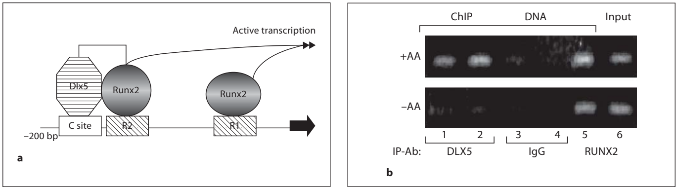
Fig. 5. In vivo binding of RUNX2 and DLX5 to chromatin sites in differentiated and undifferentiated cells. a Schematic of the proximal Bsp promoter. RUNX2 and homeodomain (DLX5) protein-binding sites are indicated. b Comparison of Bsp chromatin occupancy by RUNX2 and DLX5. Chromatin immunoprecipitation assays were used to detect RUNX2 and DLX5 bound to the proximal Bsp promoter in control (-AA) and differentiated (+AA) MC3T3-E1 clone 4 cells. Antibodies used for chromatin immunoprecipitation are indicated. Note that RUNX2 remains chromatin associated regardless of differentiated state, while DLx5 is only present in differentiated cells. c Functional interaction between R2 and C sites. 2.5-kb Bsp -luciferase reporter constructs containing all possible combinations of R1, R2 and C site mutations were transfected into MC3T3-E1 cl4 cells and grown under differentiating conditions. Note that mutation of either R2 or C is as inhibitory as mutation of both sites, while mutation of either site together with R1 gives maximal inhibition. d Protein-protein interactions between DLX5 and RUNX2. Pull-down assays with nuclear extracts from differentiated MC3T3 cells were used to show physical association between these 2 factors [Roca et al., 2005]. ChIP = Chromatin immunoprecipitation; IP-Ab = chromatin immunoprecipitation antibodies; WB = Western blot.
