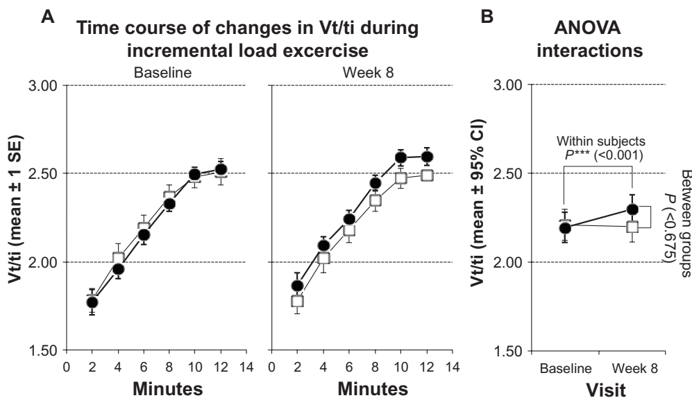
Figure 3 Measurements of mean inspiratory flow ( Vt/ti ) during incremental load test. Solid symbols \bullet : subjects with inspiratory muscle training; open symbols \square : control group. (A) Time courses of changes at baseline and after 8 weeks. Values represented as stepwise means \pm 1 standard error (SE) of the mean every 2 min; (B) results of analysis of variance (ANOVA) (repeated measurement design) representing interactions of within-subject and between-group effects.
