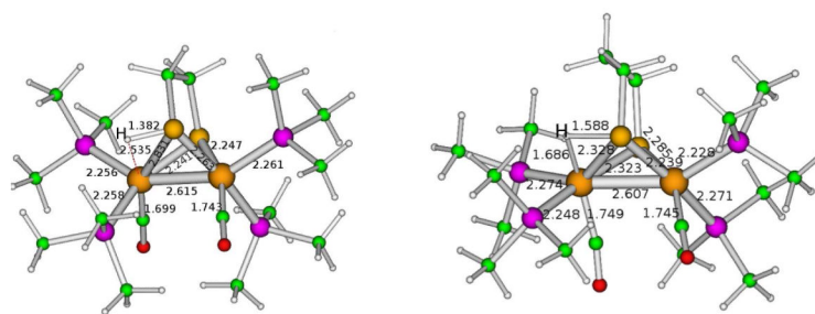
Figure 9. DFT-optimized structure of the transition state for proton transfer from S to Fe in [\text{Fe}_2(\text{Hedt})(\text{CO})_2(\text{PMe}_3)_4]^+ and [\text{Fe}_2(\text{Hpdt})(\text{CO})_2(\text{PMe}_3)_4]^+ . Note that these images are for the enantiomer of the structures shown elsewhere.
