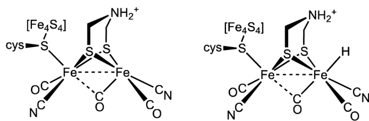
Figure 1. Structure of the active site of the [FeFe]-hydrogenase in the H ox state (left). The structure of the H red state remains uncertain - both structures are consistent with available observations. The amine cofactor is shown in the protonated form, although its protonation state is not known.
