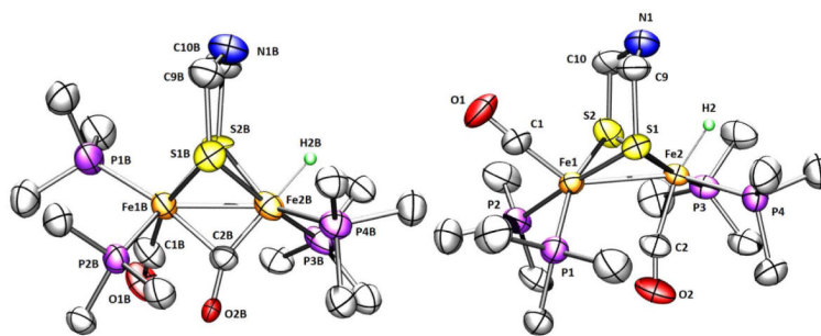
Figure 8. Structures of the cations in [\pm\text{H3}]\text{BArF}_4/[\pm\text{H3}']\text{BArF}_4 showing 50% thermal ellipsoids. Selected distances (Å) and angles (°) for [\text{H3}]^+ and [\text{H3}']^+ : Fe1B-Fe2B, 2.660(6); Fe1-Fe2, 2.659(6); O2-C2-Fe2, 152(1); O2B-C2B-Fe2B, 156(4). Fe1-C2, 2.50(1); Fe1B-C2B, 2.46(4).
