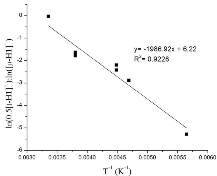
Figure 3. Temperature dependence of the product ratio [t-H1]^+ / [\mu-H1]^+ resulting from the protonation of CD_2Cl_2 solutions of 1 with H(OEt_2)_2BAr^F_4 at various temperatures.
