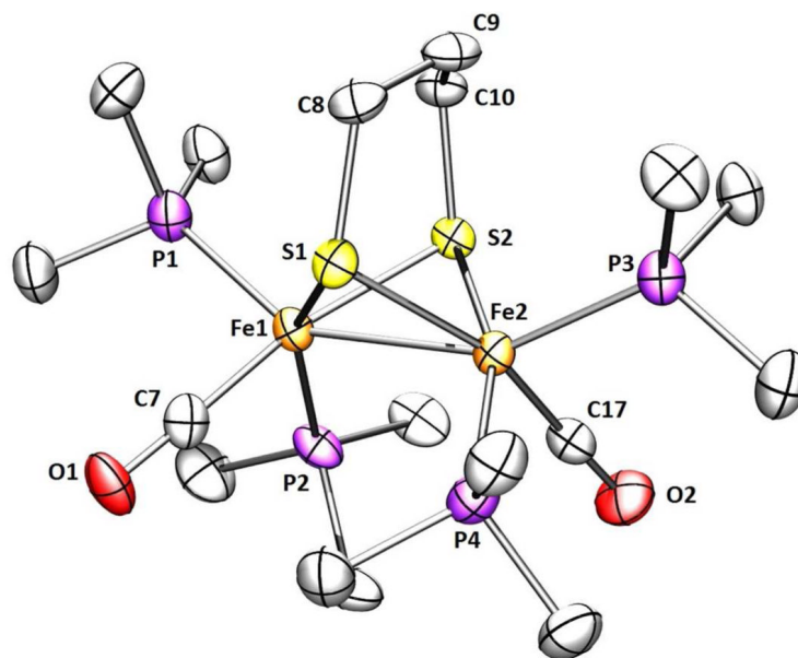
Figure 4. Structure of 2 showing 50% thermal ellipsoids. Selected distances (Å) and angle (deg): Fe1-Fe2, 2.6252(7); Fe-P avg , 2.212; S(1)-Fe(1)-Fe(2)-S(2), 109.69; P(2)-Fe(1)-Fe(2)-P(4), 90.05.
