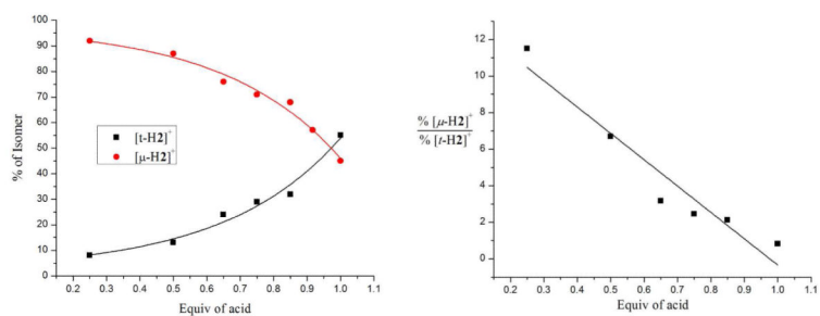
Figure 6. Product distribution for the protonation of 2 with various deficiencies of the acid \text{H}(\text{OEt}_2)_2\text{BAr}^{\text{F}_4} . The fit on the right is for 14.4[\text{Fe}_2] , = \%[\mu\text{-H}_2^+]/\%[\text{t-H}_2^+] , where
