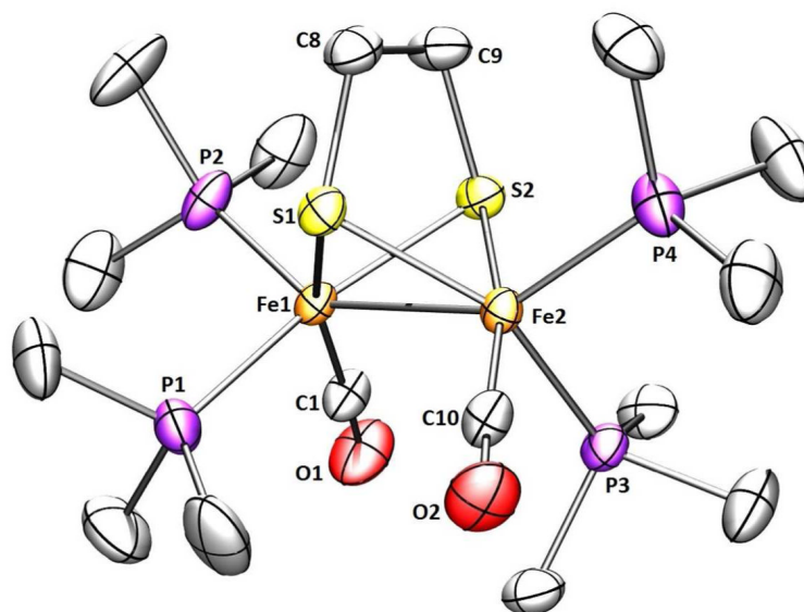
Figure 2. Structure of 1 showing 50% thermal ellipsoids. Selected distances (Å) and angles (deg): Fe1-Fe2, 2.6164(6); Fe-P avg , 2.204; S(1)-Fe(1)-Fe(2)-S(2), 103.1; P(1)-Fe(1)-Fe(2)-P(3), 94.24.
