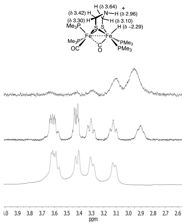
Figure 7. ^1\text{H} NMR spectra in the adt region of a \text{CD}_2\text{Cl}_2 solution of [\text{t-H3}]^+ . Top is the result of 1-D nOe experiment upon irradiation at \delta -2.11 . Middle and bottom: spectra before and after addition of \text{D}_2\text{O} , respectively (the Fe-H signal also vanishes). The shoulder on the \delta 3.6 multiplet arises from [\text{t-H3}']^+ .
