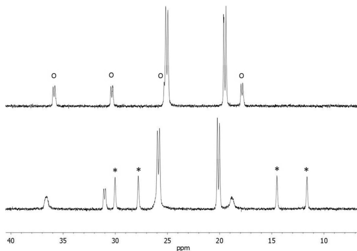
Figure 5. ^{31}\text{P}\{^1\text{H}\} NMR spectra for protonation of \text{Fe}_2(\text{pdt})(\text{PMe}_3)_4(\text{CO})_2 with one equiv of \text{H}(\text{OEt})_2\text{BAr}^{\text{F}_4} , starting at -90\text{ }^\circ\text{C} (bottom). The same solution at -60\text{ }^\circ\text{C} is shown above. In the -90\text{ }^\circ\text{C} spectrum, the four singlets assigned to a S -protonated species ( [\text{S-H2}]^+ ) are indicated with *. Signals assigned to [\text{t-H2}]^+ are indicated with o. The two doublets are assigned to [\mu\text{-H2}]^+ .
