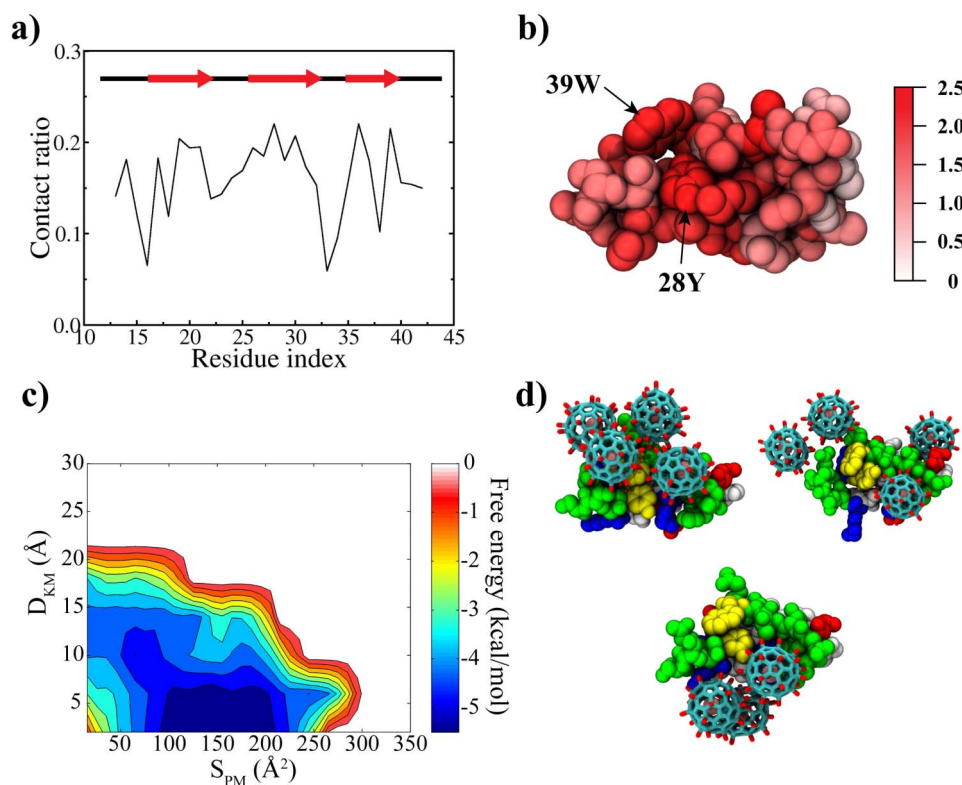
Figure 2 | (a) Site-specific contact ratio of WW domain, where the contact ratio of a residue was obtained by counting the number of frames of the residue in contact with Gd@C 82 (OH) 22 over all time frames; (b) Residues involved in contact with Gd@C 82 (OH) 22 ; (c) The binding free energy surface, where D KM is the minimum distance between Gd@C 82 (OH) 22 and the signature residues (Y28 and W39) of the WW domain and S PM is the contacting surface area; and (d) Representative binding modes found in the global minimum. Yellow: key residues, white: hydrophobic, green: non-charged polar, red: negatively charged and blue: positively charged residues.
