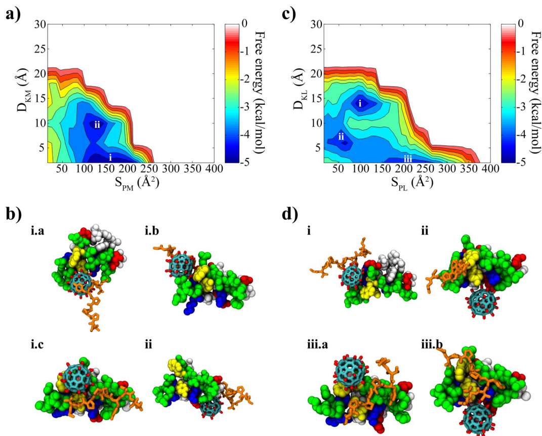
Figure 4 | (a) Binding free energy landscape between WW domain and \text{Gd@C}_{82}(\text{OH})_{22} and (b) representative structures found in local energy minima. (c) Binding free energy landscape between WW domain and PRM and (d) representative structures found in local energy minima. D and S of two axes in the free energy diagrams indicate distance and contact area, respectively. The subscripts P, K, L and M represent protein, key residues, PRM ligand and \text{Gd@C}_{82}(\text{OH})_{22} , respectively. The local energy minima are rank-ordered starting from the global minimum in the (a) and (c).
