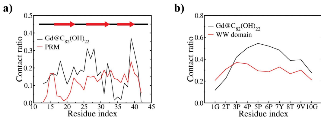
Figure 3 | (a) Site-specific contact ratio of WW domain by \text{Gd@C}_{82}(\text{OH})_{22} and PRM and (b) site-specific contact of PRM by \text{Gd@C}_{82}(\text{OH})_{22} and WW domain.
