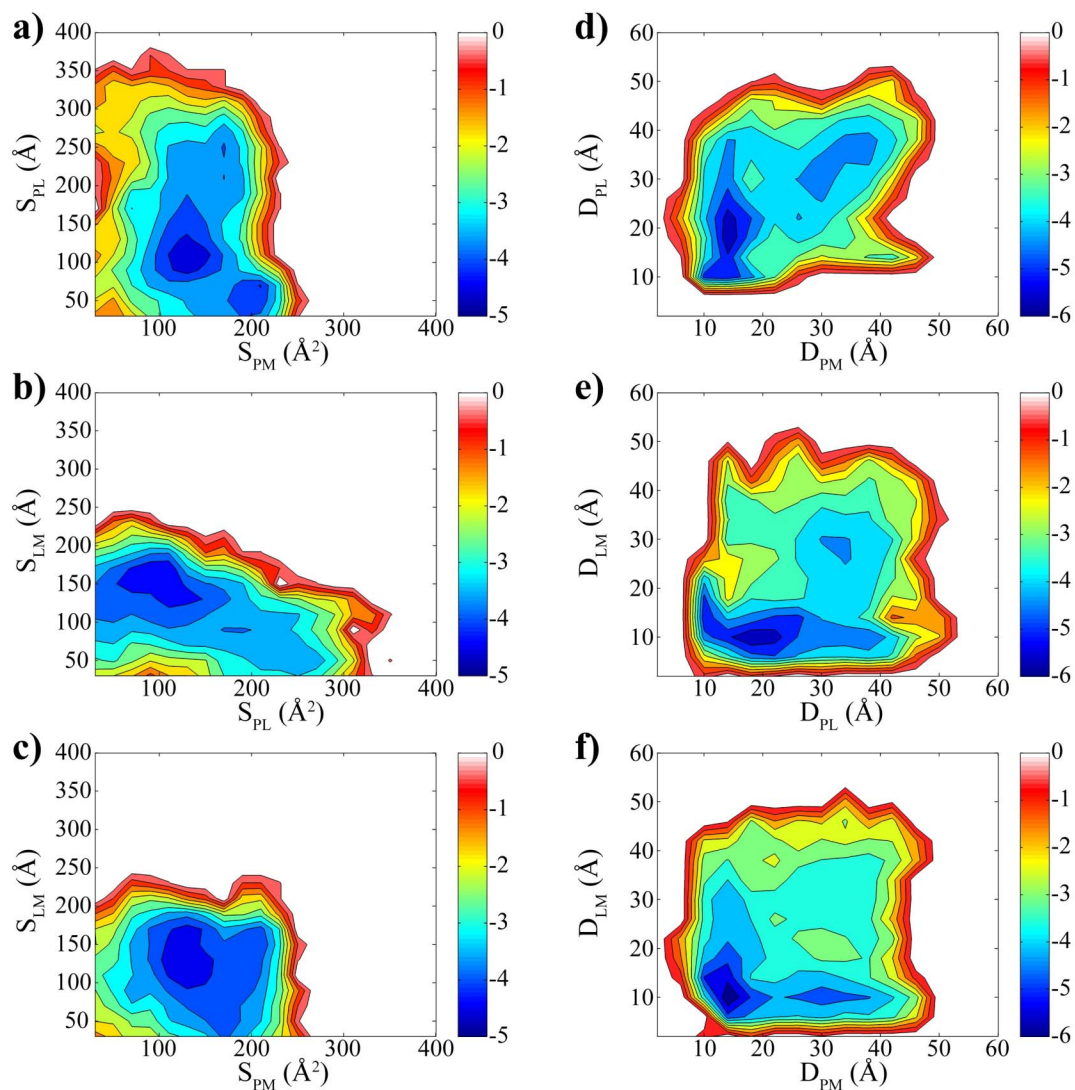
Figure 5 | Relative binding preference. (a) and (d) Binding preference for WW domain toward PRM and \text{Gd@C}_{82}(\text{OH})_{22} . (b) and (e) Binding preference for PRM toward WW domain and \text{Gd@C}_{82}(\text{OH})_{22} . (c) and (f) Binding preference of \text{Gd@C}_{82}(\text{OH})_{22} toward WW domain and PRM. The contact areas were used for panel (a), (b) and (c) and the centre-of-mass distances for panel (d), (e) & (f).
