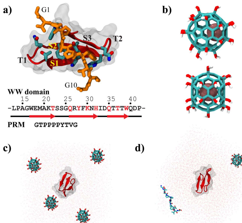
Figure 1 | (a) Complex structures of the WW domain and proline rich motif (PRM); (b) Molecular structure of Gd@C 82 (OH) 22 ; (c) Initial simulation system for the intrinsic binding dynamics of Gd@C 82 (OH) 22 on the WW domain; and (d) Initial system for the inhibitory dynamics of Gd@C 82 (OH) 22 in competition with PRM.
