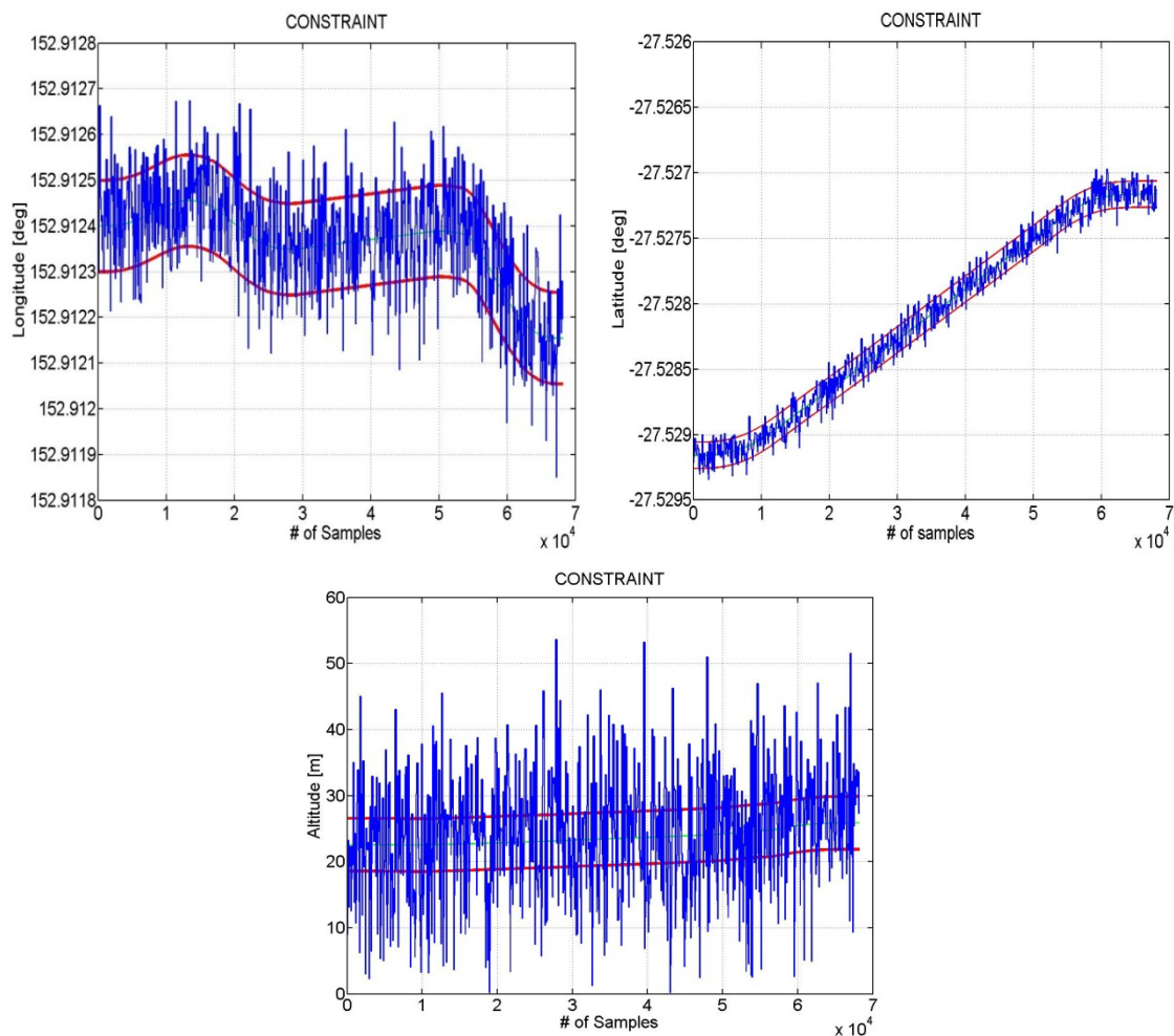
Figure 8. Example of constraints on position. The boundaries of the street are shown (red lines) and the user position has been approximated as affected by a white noise (blue).
