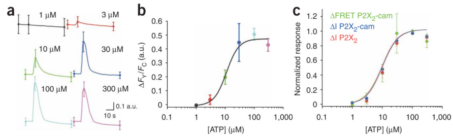
Figure 2. Concentration-dependent ATP-evoked FRET changes for P2X 2 -cam channels expressed in HEK cells. (a) Representative F_Y/F_C traces for puff application of the indicated ATP concentrations. (b) Concentration-response curves for ATP-evoked changes in F_Y/F_C . (c) Normalized concentration-response curves for ATP-evoked changes in F_Y/F_C , currents for P2X 2 -cam receptors and currents for wild-type P2X 2 receptors.
