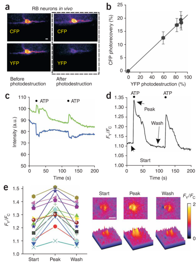
Figure 6. In vivo FRET experiments for P2X 2 -cam channels. (a,b) Representative images and plot of FRET efficiency of P2X 2 -cam receptors in RB neurons in vivo . (c,d) Fluorescence intensity and F_Y/F_C data for ATP-evoked FRET changes for P2X 2 -cam receptors in RB neurons. (e) Left, scatter graph showing data from all fish that did not move. Right, FRET images of the ATP-evoked changes. Scale bars, 10 \mu m (a,e) .
