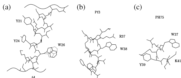
Fig. 9. Orientations of tryptophan and tyrosine residues in the protein subunits of bacteriophages: fd, Pf3 and PH75. The Trp 26 orientation as initially proposed in the model of Marvin et al. 24 is represented by dotted lines in the fd illustration. The orientation determined experimentally by polarized Raman spectroscopy is also shown (solid lines). 33
