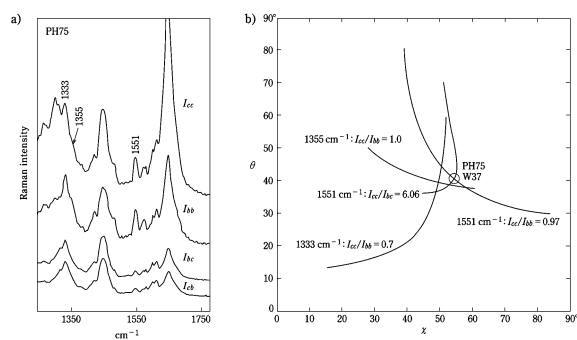
Fig. 8. (a) Polarized I_{cc} , I_{bb} , I_{bc} , and I_{cb} Raman spectra ( 1300\text{--}1750\text{ cm}^{-1} ) obtained from an oriented fiber of PH75 that was excited at 532\text{ nm} . (b) Contour maps in \theta, \chi -space showing I_{cc}/I_{bb} values for the 1333 , 1355 and 1551\text{ cm}^{-1} Raman bands of Trp 37. The contour line is also shown for the ratio I_{cc}/I_{bc} of the 1551\text{ cm}^{-1} band. On the basis of these results the Eulerian angles ( \theta, \chi ) that define the orientation of the Trp 37 indolyl plane with respect to the virion axis are: \theta = 45^\circ and \chi = 59^\circ (denoted by the open circle at the center of the plot).
