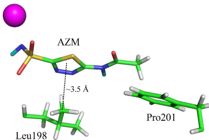
Figure 5. Ball-and-stick representation of the AZM weak hydrophobic interactions within the active site of HCA II. D (cyan) and H (white - positions calculated) atoms. Zinc is shown as a magenta sphere.
