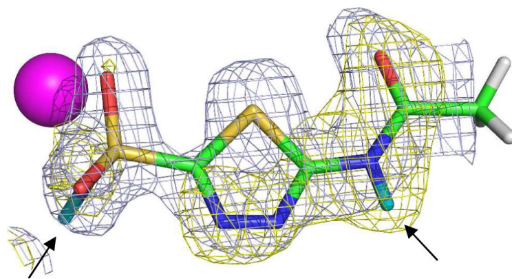
Figure 2. Stick representation of AZM bound to HCA II. Zinc is shown as a magenta sphere, D atoms are in cyan (indicated by arrows), H atoms in white (positions calculated). The nuclear density map is shown in yellow and is contoured at 1.5 \sigma , the electron density map is shown in blue and is contoured at 2.0 \sigma .
