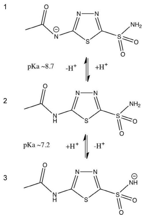
Figure 1. Ionization and \text{pK}_a of acetazolamide (AZM) in water. These different charged states represent the relevant forms that may bind HCA II under physiological conditions. Figure was drawn with ChemDraw (Perkin Elmer) and adapted from Supuran & Winum, 2009. 10
