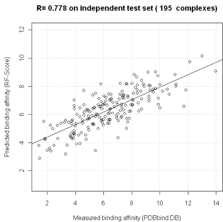
Figure 3. RF-Score predicts the test data with high accuracy (Pearson correlation coefficient R=0.778 and RMSE=1.58 ).
