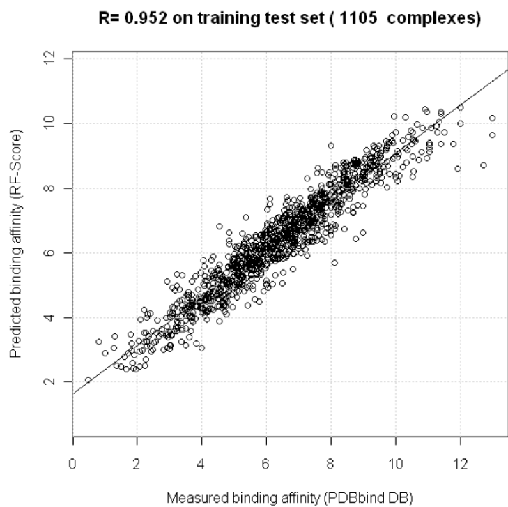
Figure 1. RF-Score reproduces its training data with very high accuracy (Pearson correlation coefficient R=0.952 and RMSE=0.74 ).
